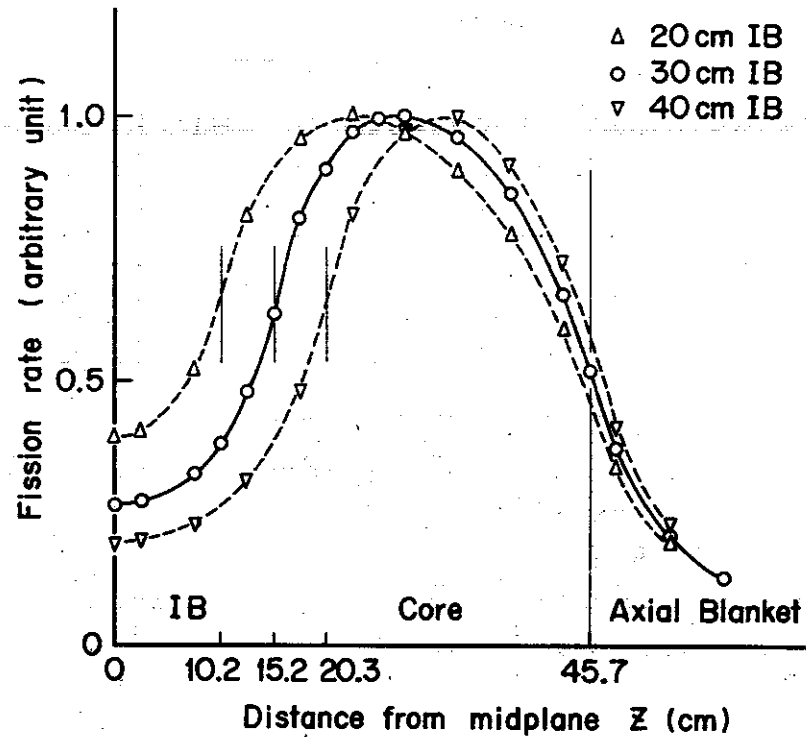
Fig. 9 Axial fission rate distributions of depleted U mfc measured in FCA Assembly VII-3.
