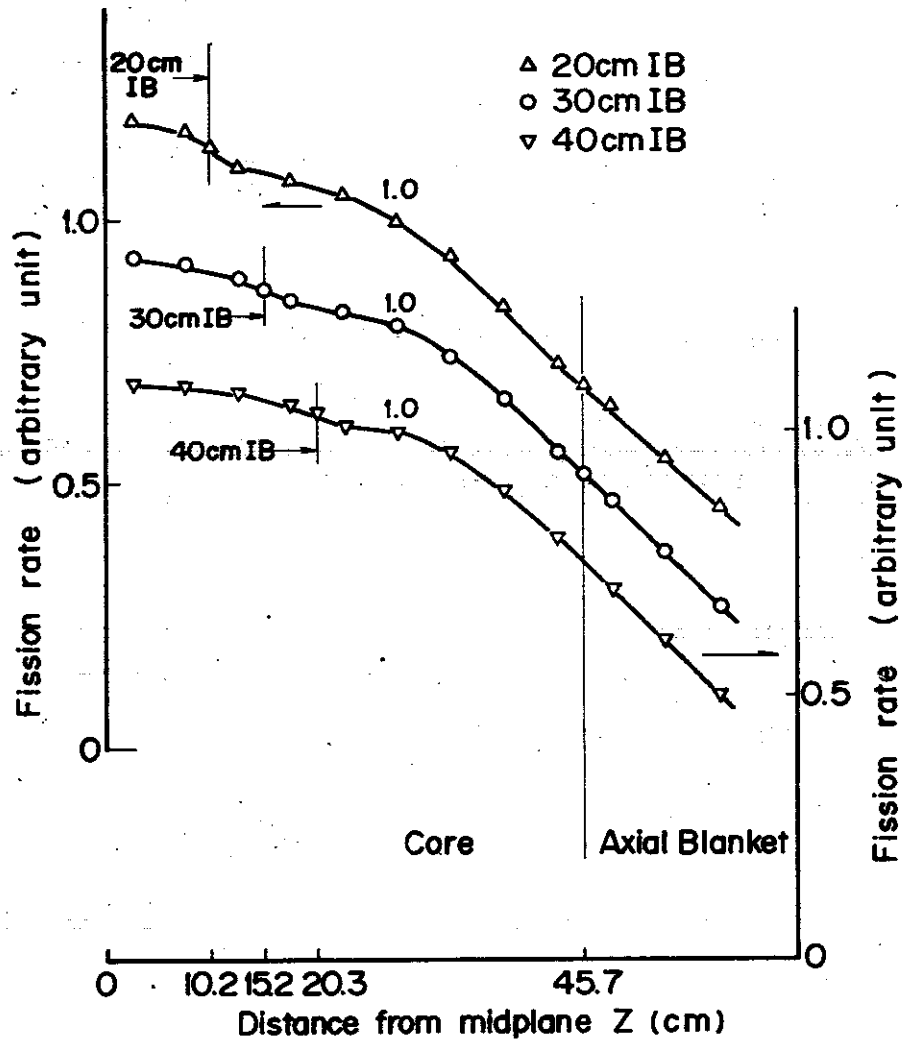
Fig. 8 Axial fission rate distributions of Pu-239 mfc measured in FCA Assembly VII-3.
