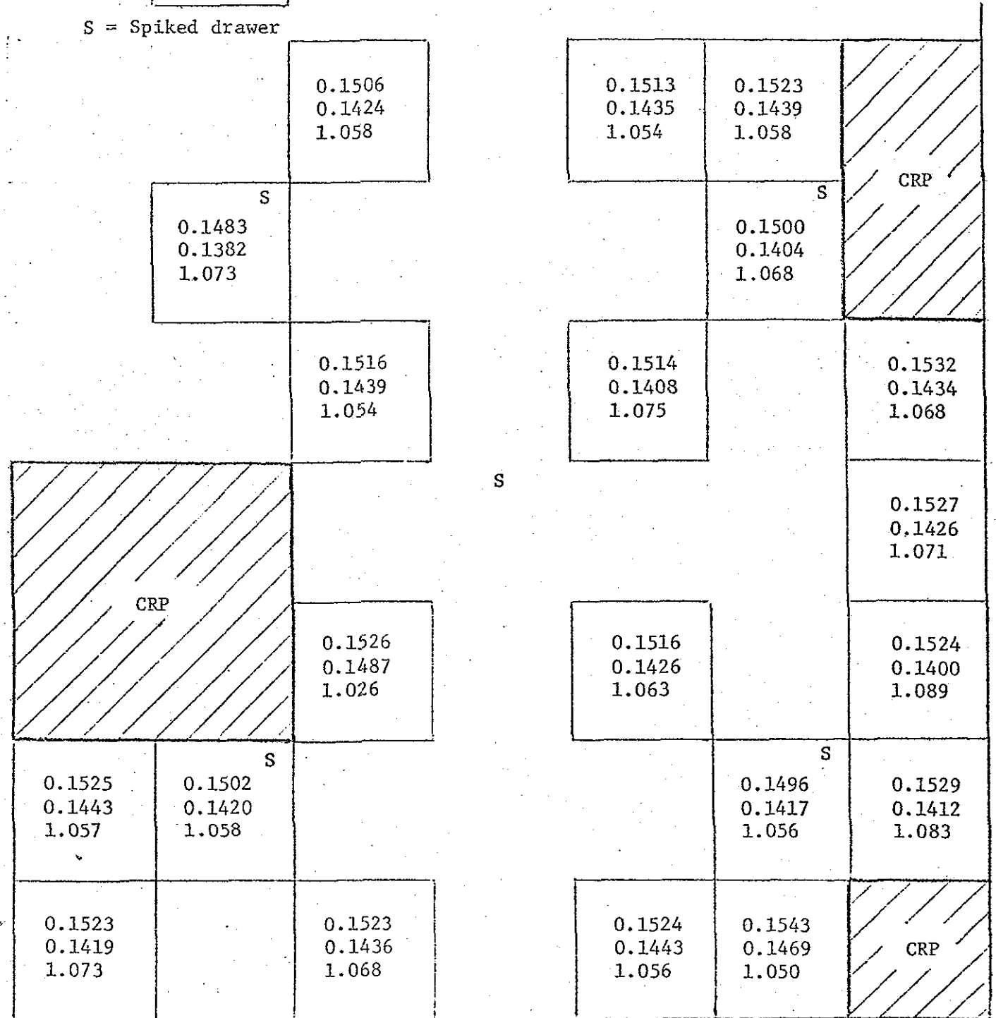
Fig. 1 Variation of C_8/F_9 Near the Center of ZPPR-4/1
