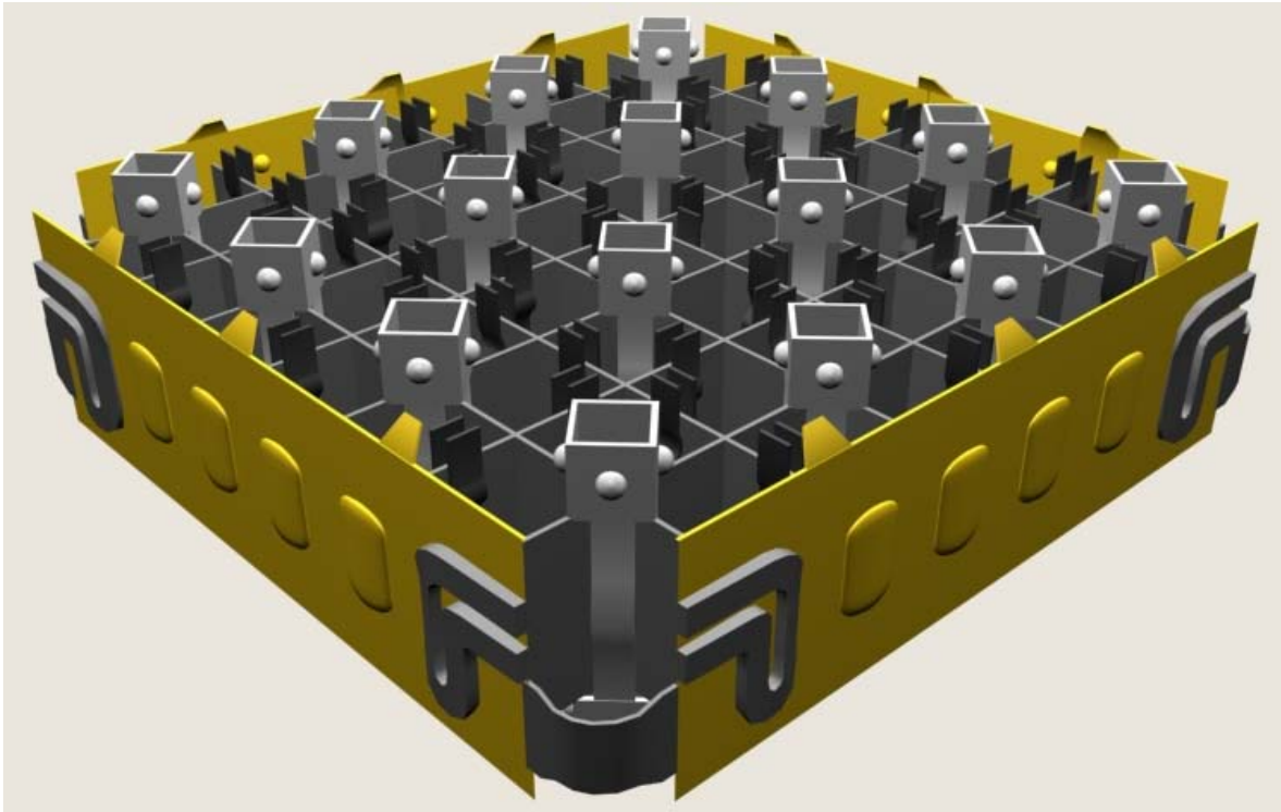
Figure 3.5.9 Grid Spacer – 3D View
