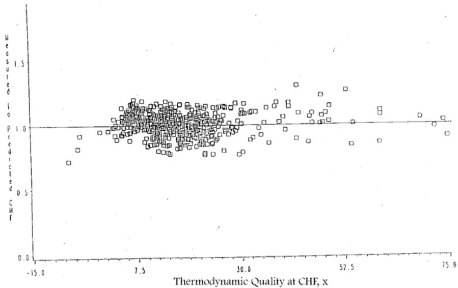
Figure A.4 Example of Measured to Predicted CHF versus Quality
