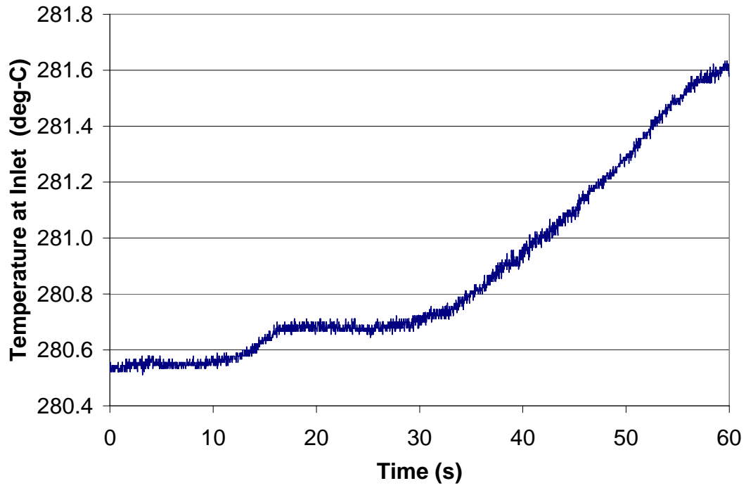
Figure 4.2.4 Turbine Trip Transient Void Distribution Experimental Boundary Conditions, Assembly Type 4 –Inlet Temperature
