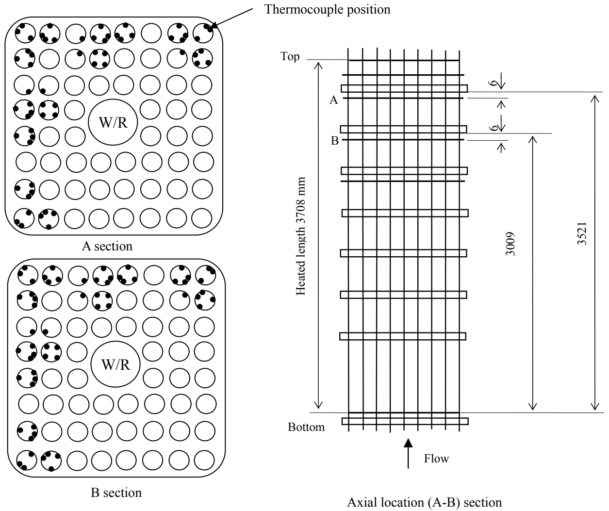
Figure 2.5.4 Location of Thermocouples for Critical Power Measurement (C2B)
