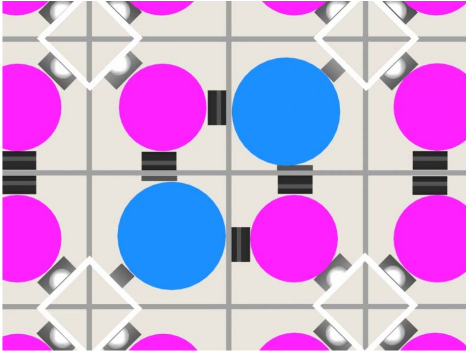
Figure 3.5.5 Grid Spacer – Central View
