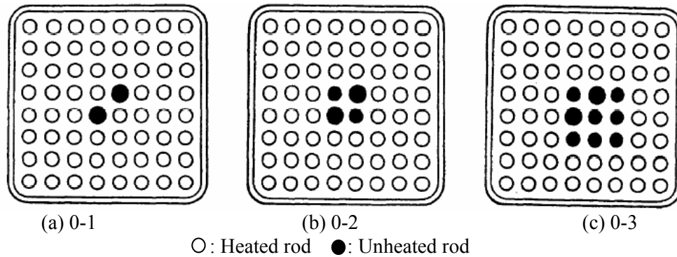
Figure 3.2.1 Unheated Rods Arrangements in Test Assembly Type 0
