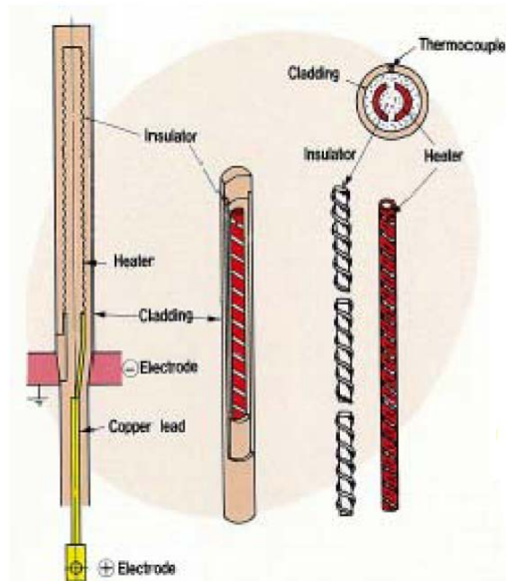
Figure 3.3.1 Cross Sectional View of Heater Rod
