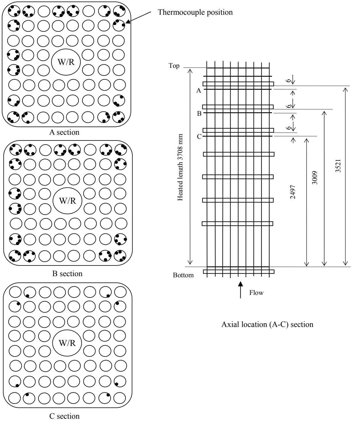
Figure 2.5.3 Location of Thermocouples for Critical Power Measurement (C2A)
