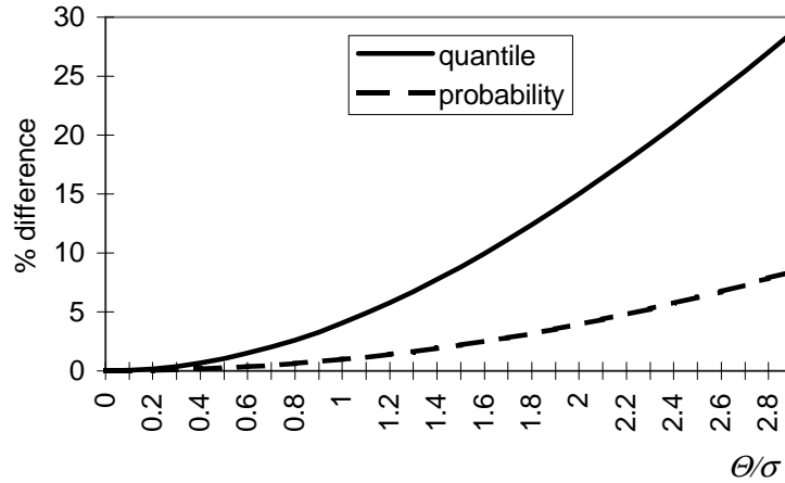
Figure F.1. Percentage difference between quantiles \gamma and \gamma_G as well as (1-\varepsilon) and the (1-\varepsilon') given by Equation 4 for various values of \theta/\sigma . ( \varepsilon = 0.05 .)
