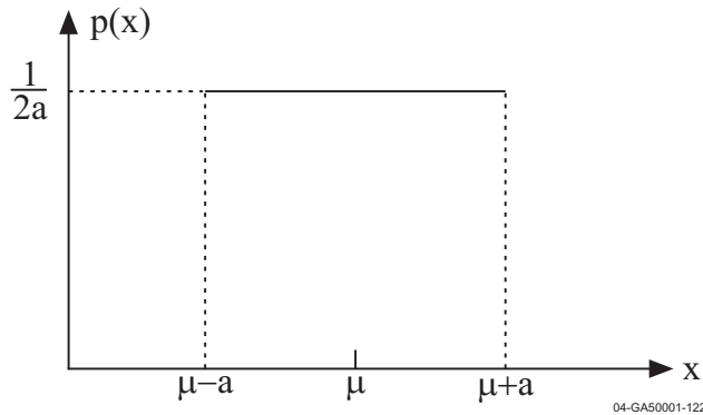
Figure G.1. Probability Density Function p(x) for Variable x , Assumed to Be Uniformly Distributed between \mu-a and \mu+a .
