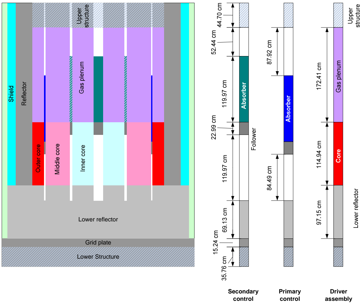
Figure 3. RZ Geometry Model of 1000 MWt ABR Oxide Core
