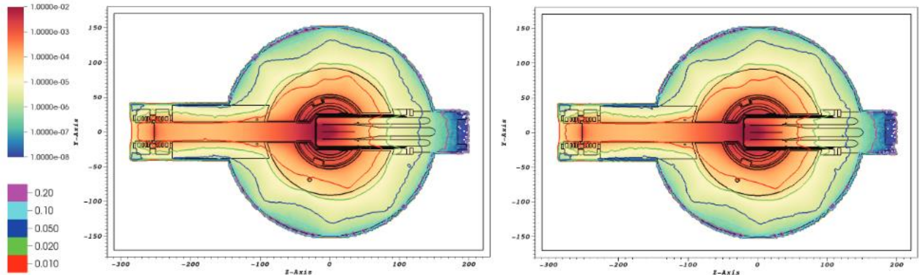
SNS geometry translated by mcnp2cad (MCNP geometry left) and DAG-MCNP geometry right
