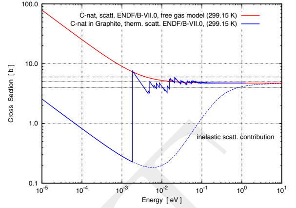
FIG. 38 Elastic scattering cross-sections of carbon at room temperature (free gas model) vs. thermal scattering cross-sections of carbon in graphite at room temperature.
