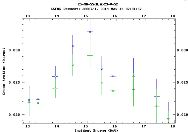
FIG. 4 Sample rescaling of the ^{55}\text{Mn}(n, \alpha) from Viktor Zerkín’s EXFOR-Web (EXFOR, 2015) on the IAEA nuclear data services website (IAEA, 2015).
