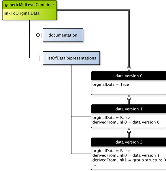
FIG. 7 Sketch of a generic mid-level container. Note the use of links to represent what data were derived from what other data and to denote which data set were the original. This motif is used repeatedly throughout the hierarchy. Note that the originalData and <derivedFrom> are redundant in this example; we really only need a <derivedFrom> element to denote what is derived and what is original.
