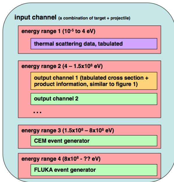
FIG. 21 Gluing together different models from different energy regions.
