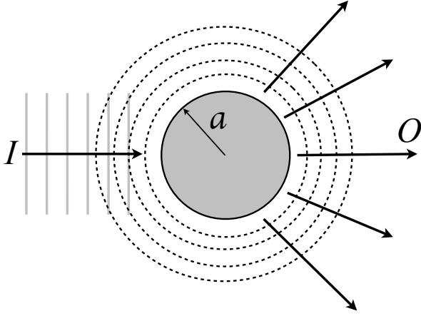
FIG. 16 A cartoon representation of R matrix theory. We first divide the universe into inside a box and out. Inside the box is the reaction zone, that we have little chance of modeling correctly without a lot of work. Outside the box we write all incoming and outgoing relative two-body scattering states in a basis of analytic wave functions, usually taken to be free ones. We then match wave functions on the box boundary.
