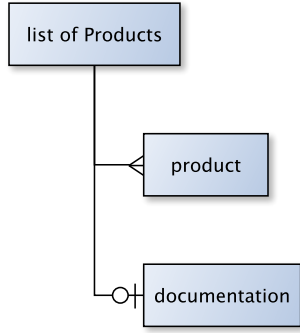
FIG. 9 Common arrangement of a product list element such as <reactionProducts> , <decayProducts> or <orphanedProducts> .
