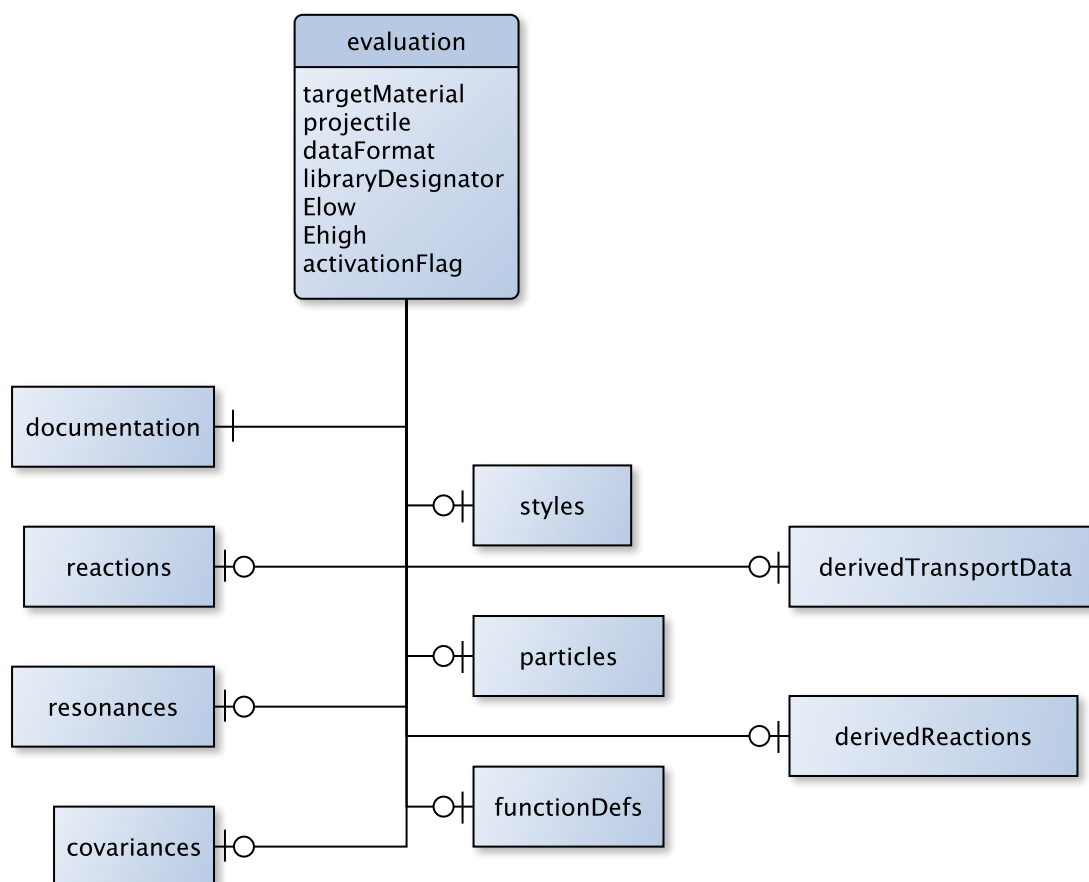
FIG. 12 Top level arrangement of an <evaluation> element. Only the documentation element is required in an <evaluation> , but <reactions> , <resonances> , and <covariances> are expected in nearly all (neutron induced) reaction evaluations. The <styles> , <particles> and <functionDefs> elements are used primarily to override or (re)define default behaviors. Finally, the <derivedReactions> and <derivedTransportData> elements are nearly exclusively for processed data.
