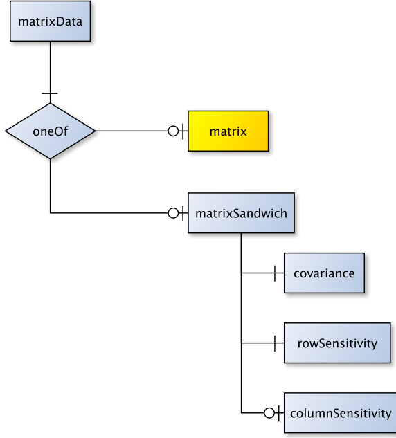
FIG. 28 Arrangement of parts of a <matrixData> element. The matrix may be stored either in low-level <matrix> container or as a “matrix sandwich” (see Eq. (22) below).
