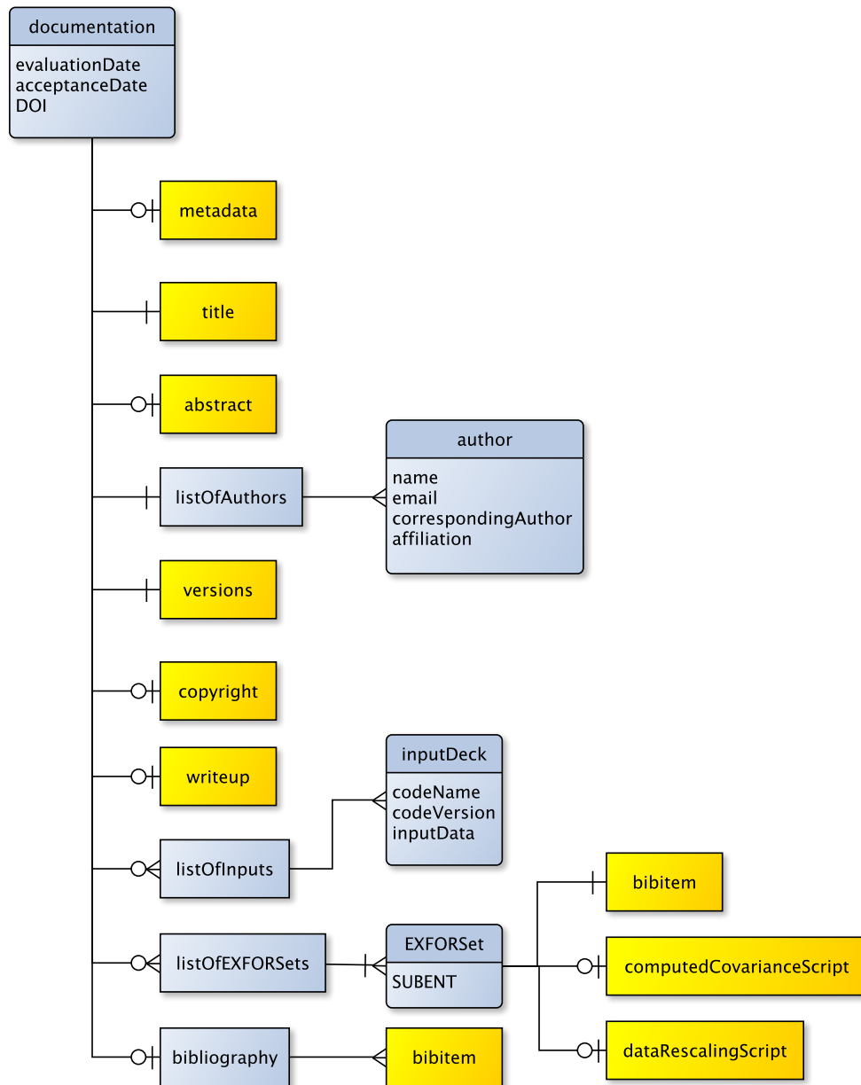
FIG. 2 Basic structure of a <documentation> element.
