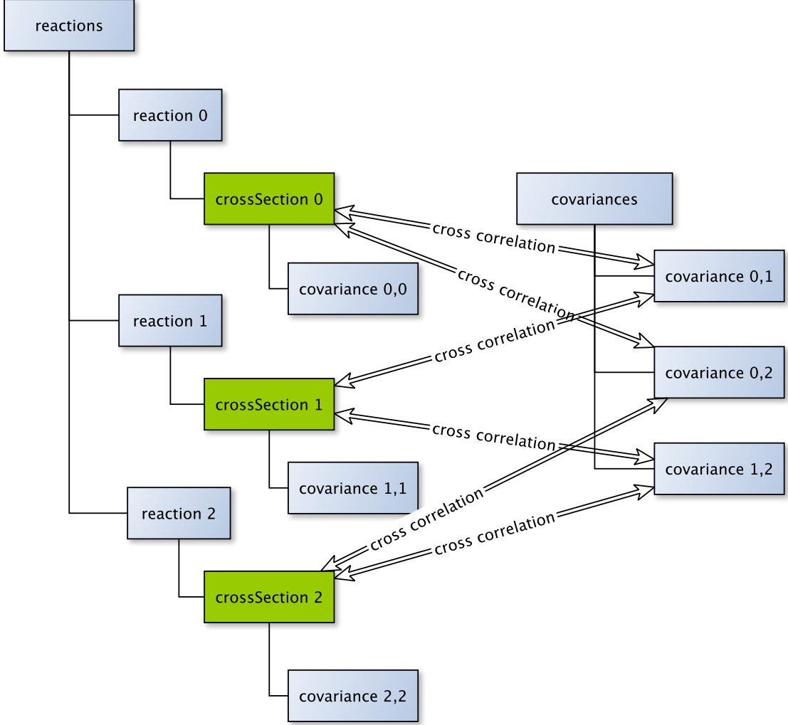
FIG. 26 Coupling between reaction data and the corresponding covariance. This figure is a continuation of the example in Fig. 25, highlighting the links between a data element and the cross-covariances associated with it.
