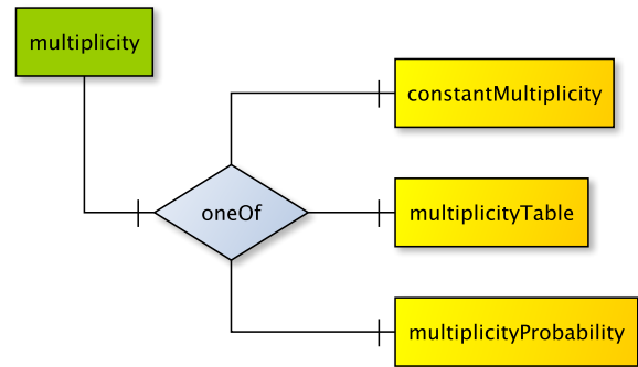
FIG. 11 Overview of a <multiplicity> element.
