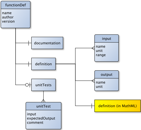
FIG. 39 The <functionDef> Outline of the functionDef scheme for prototyping new functional forms and interpolation schemes.
