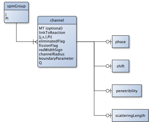
FIG. 17 Our channel element.
