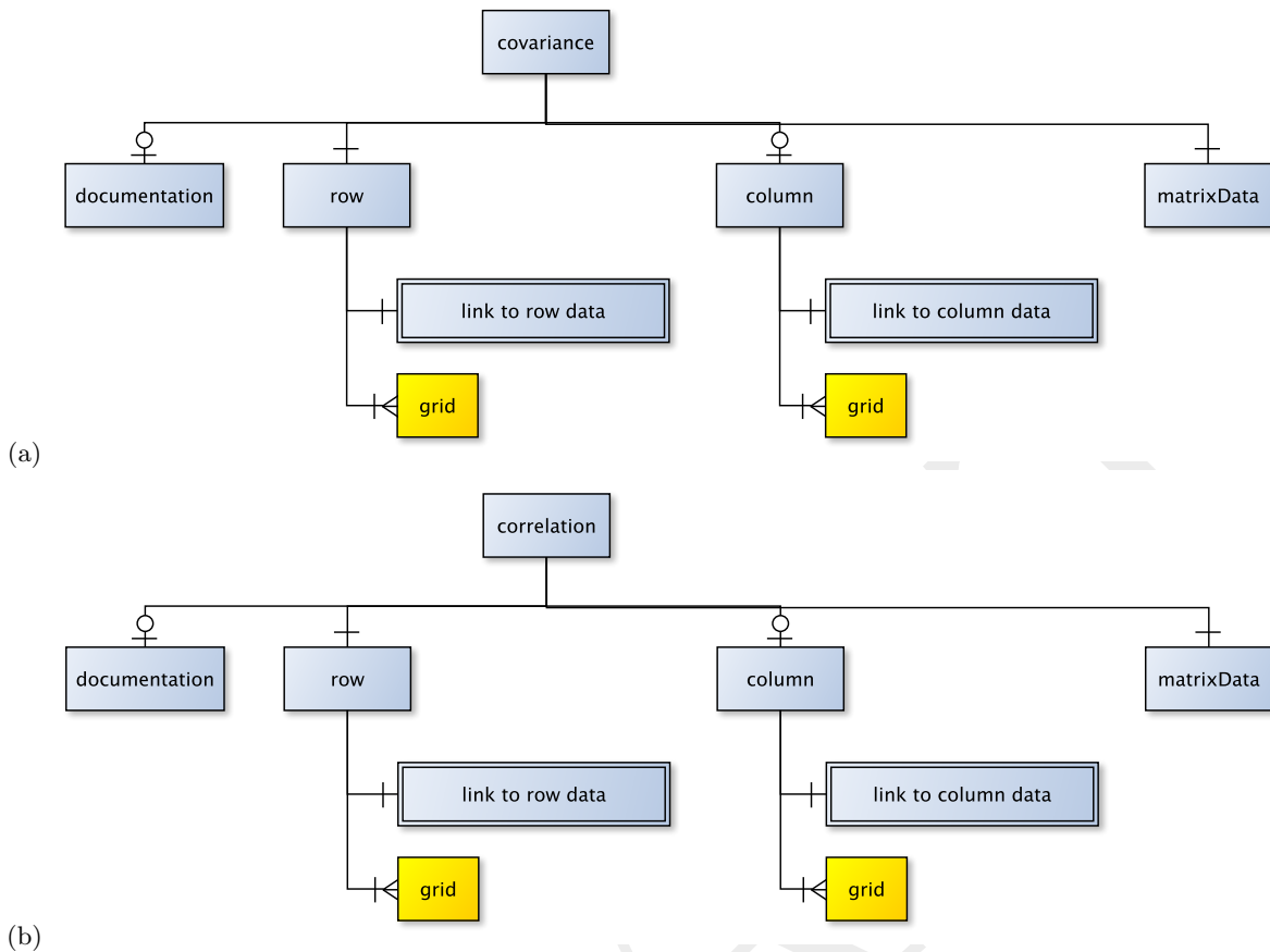
FIG. 27 The <covariance> and <correlation> elements. As they share identical components, but have very different meanings, the element name must most likely be used to distinguish them.
