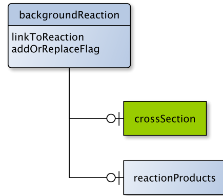
FIG. 19 Overview of elements to repair or amend cross section and other reaction data.
