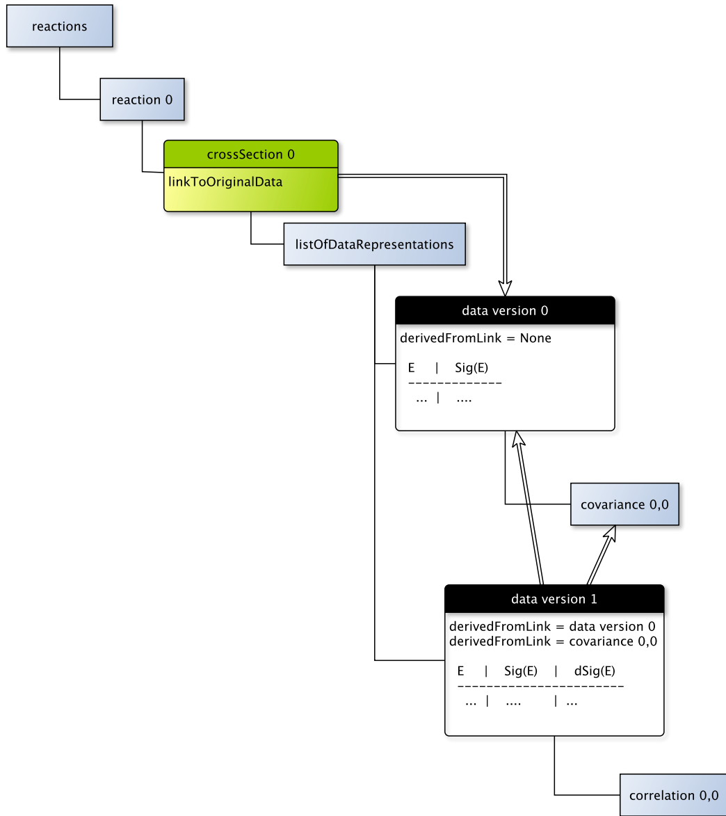
FIG. 8 An illustration of uncertainty in a data set, but derived from original data and a covariance. The coupling between reaction data and the corresponding covariance is handled through use of hyperlinks.
