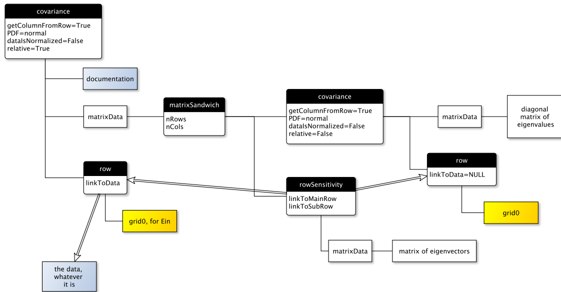
FIG. 32 Illustrating the use of the <sensitivityMatrix> approach to compress a covariance matrix using the principal components of the covariance determined from an eigenvalue decomposition.
