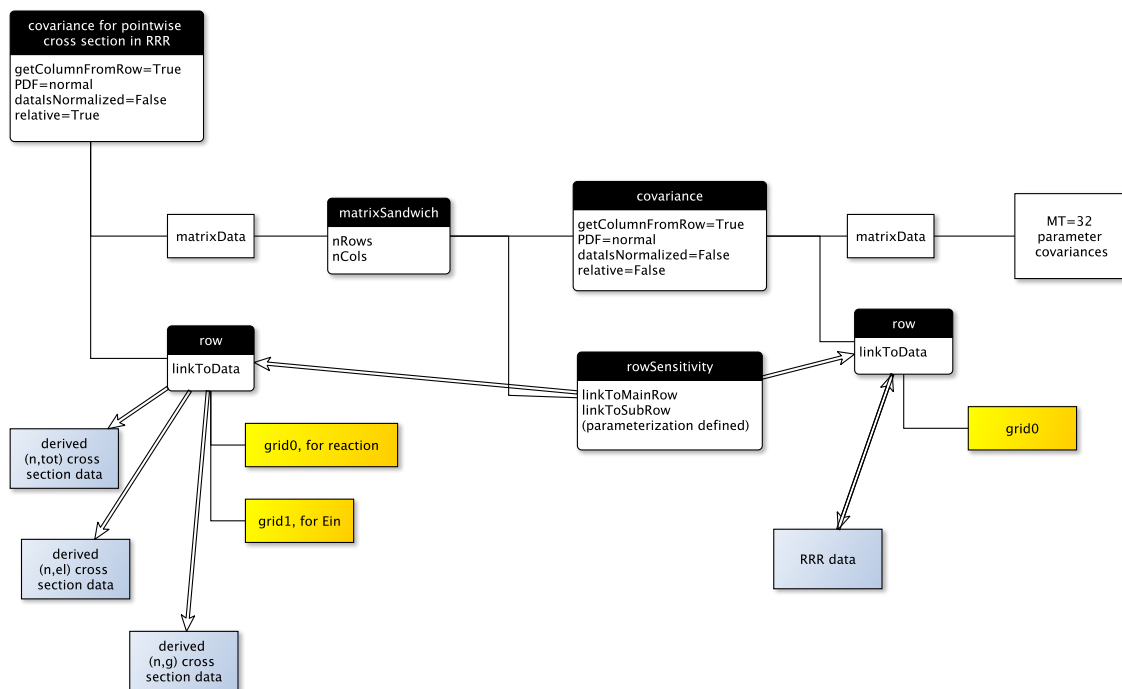
FIG. 33 Illustrating the storage of resonance covariance data. This is our approach to the ENDF format's MF=32.
