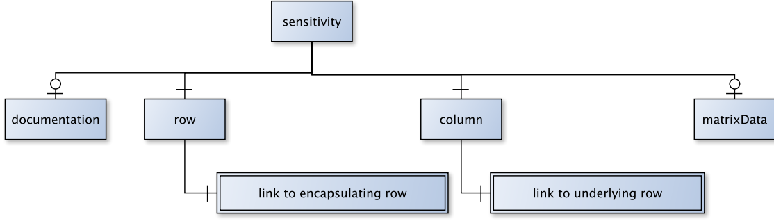
FIG. 30 The <sensitivityMatrix> element which connects the small matrix inside a “matrix sandwich” to the external covariance matrix in Eq. (22).
