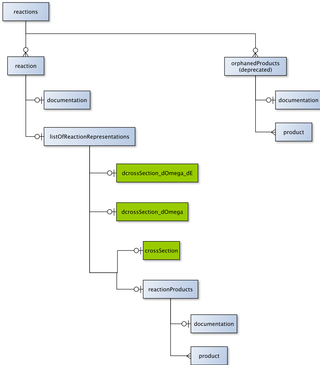
FIG. 13 A possible arrangement of inclusive and exclusive reactions in the <reactions> element. Note that there are three options for the double differential cross section data: a) store d\sigma(E)/dE'd\Omega , b) store d\sigma(E)/d\Omega if the outgoing energy is fixed by kinematics or c) store both \sigma(E) and P(E', \mu|E) separately. In some cases the total cross section \sigma(E) is not defined and one must use one of the other options.
