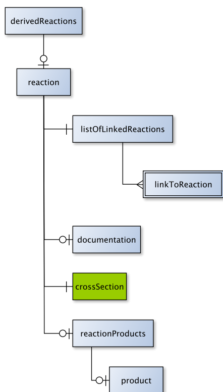
FIG. 14 Layout of the <derivedReactions> element.
