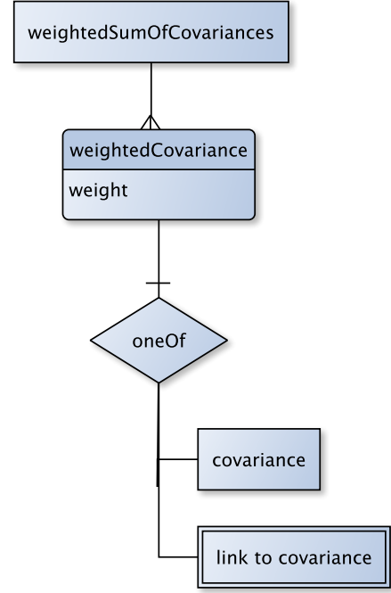
FIG. 29 The <weightedSumOfCovariances> element.
