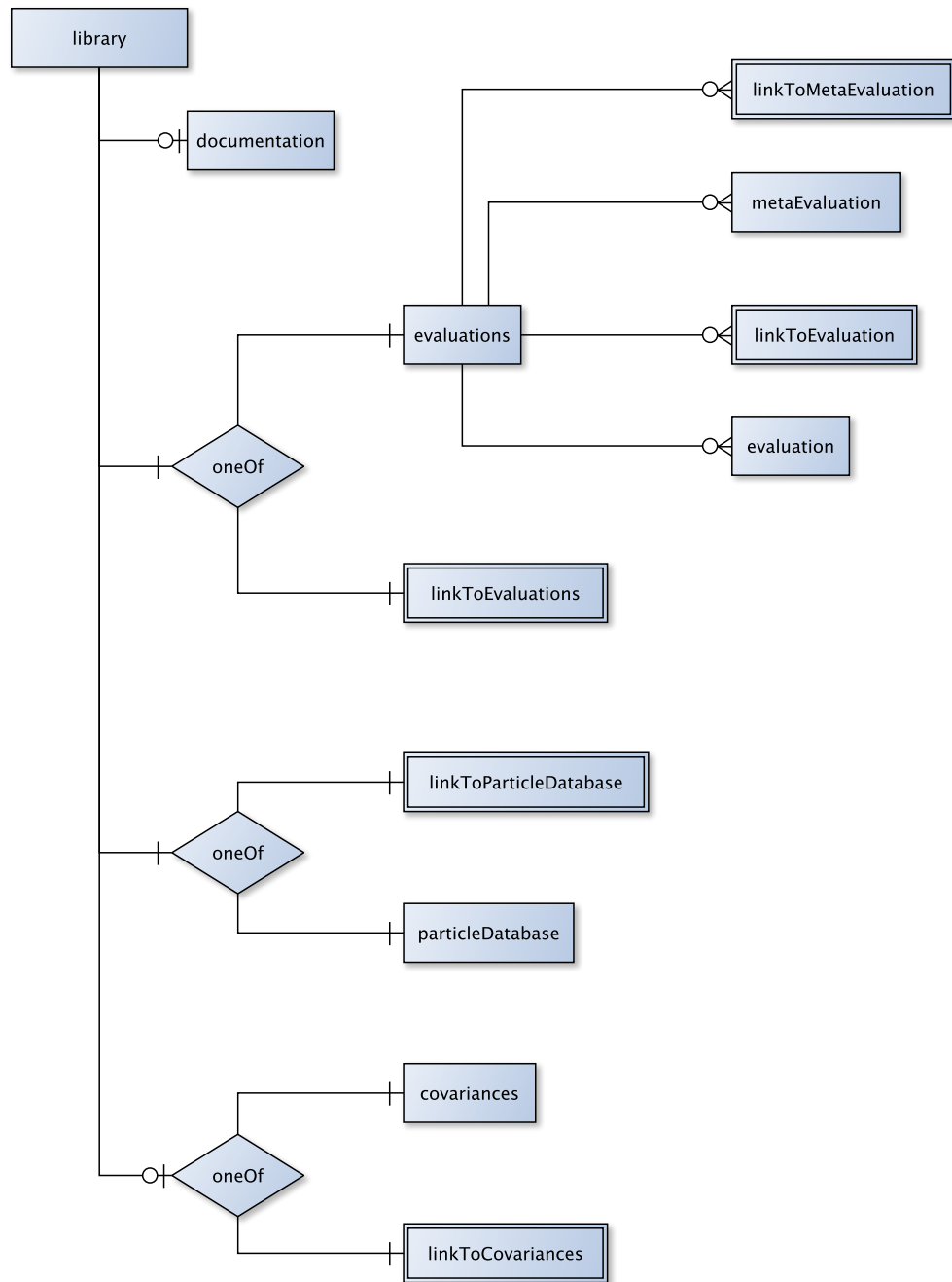
FIG. 20 Grouping evaluations, covariances and/or particle properties.
