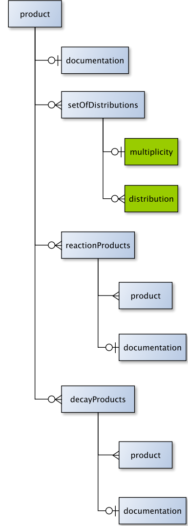
FIG. 10 Overview of a <product> element.
