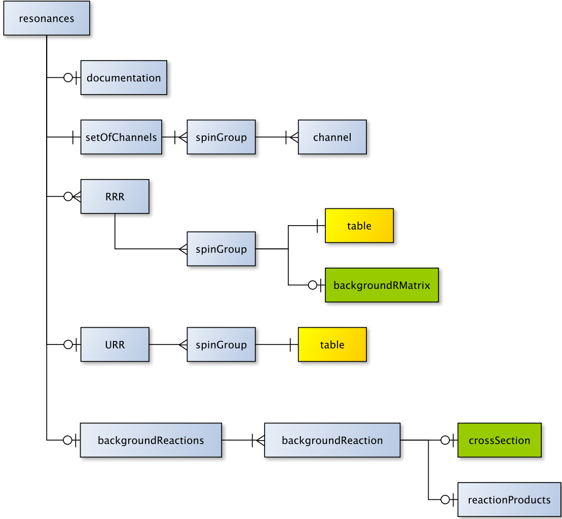
FIG. 15 Our proposed resonance data hierarchy.
