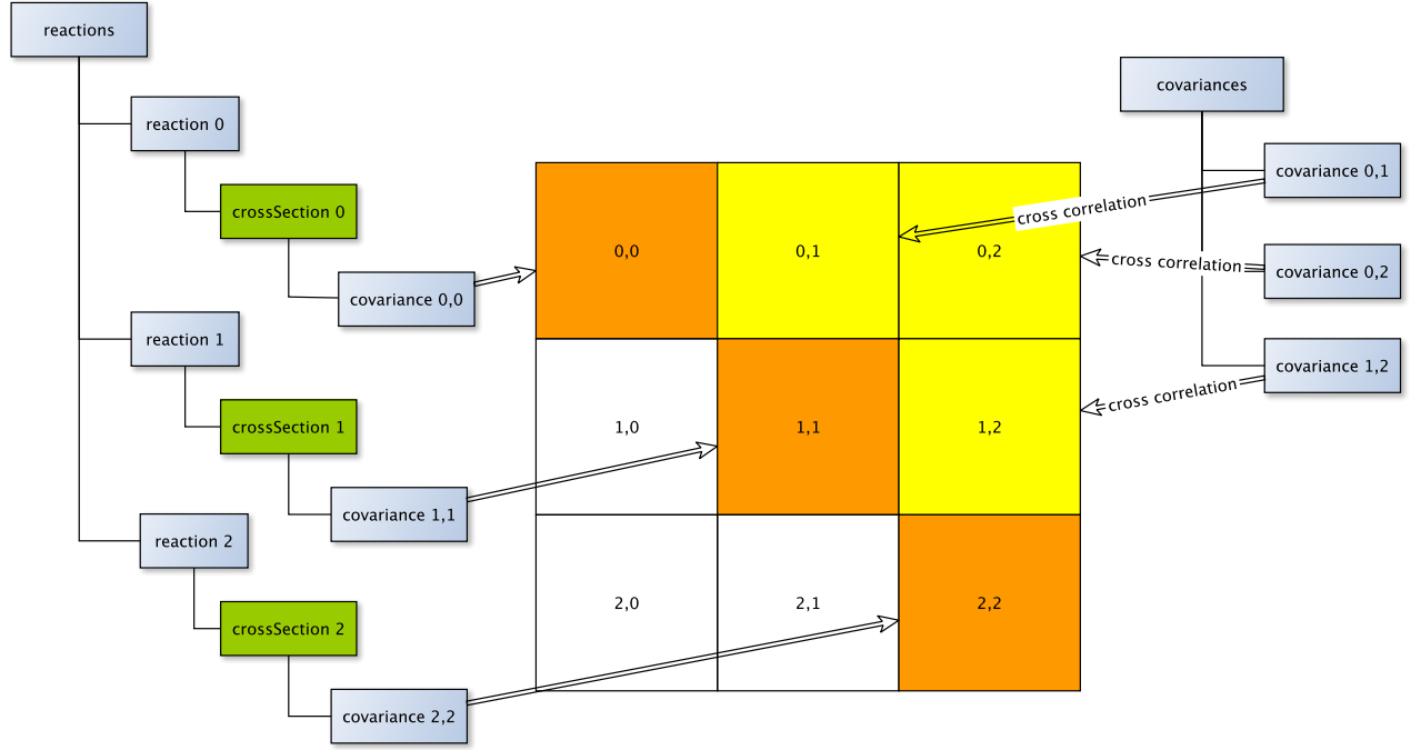
FIG. 25 Relationship of self-covariance and cross-reaction covariances, illustrating where they are to be stored in data files. The central covariance matrix is divided up into rectangular blocks, corresponding to different observables. The self-covariances are stored with the data elements in the tree on the left and the cross-covariance parts are stored in a separate list on the right.
