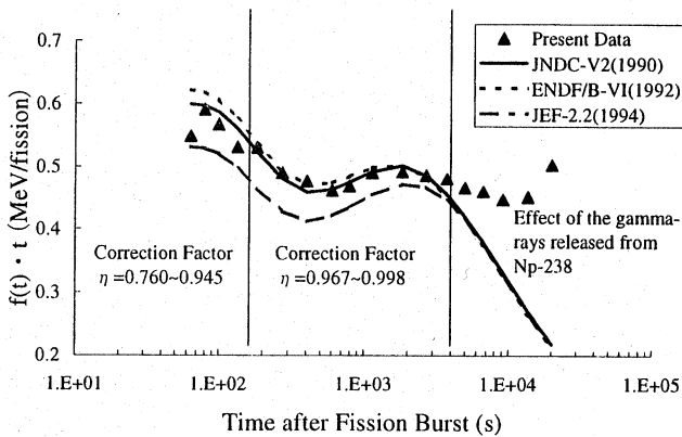
Fig. 4 Gamma Fission Burst Decay Heat for Np-237
