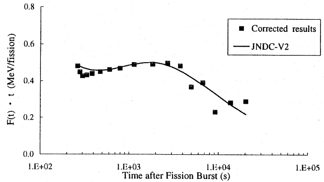
Fig.6 Np-237 Gamma Decay Heat Corrected for Gamma-rays of Np-238
