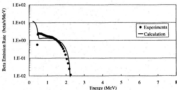
Fig.9 Comparison between Measured and Calculated Sr-90+Y-90 Beta-ray Spectrum
