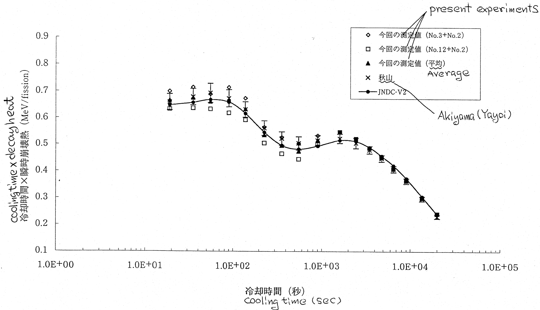
図4-6-4 U-235 \gamma 線瞬時照射崩壊熱 (10秒照射結果+100秒照射結果) U-235 Decay Heat \gamma -ray Component, Burst Fission
