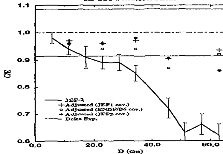
Figure 2: C/E values, with the corresponding M-C statistical error, for the reaction rates calculated using JEF-2. The linear theory based estimated C/E for the adjusted JEF2 cross-sections, using different covariance matrices, are shown as well.
