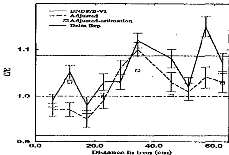
Figure 1: C/E values for the reaction rates calculated using ENDF/B-VI original and adjusted cross-sections. M-C statistical error is shown as well. "Estimation" are the C/E values calculated by the adjustment code on the basis of the linear theory.
