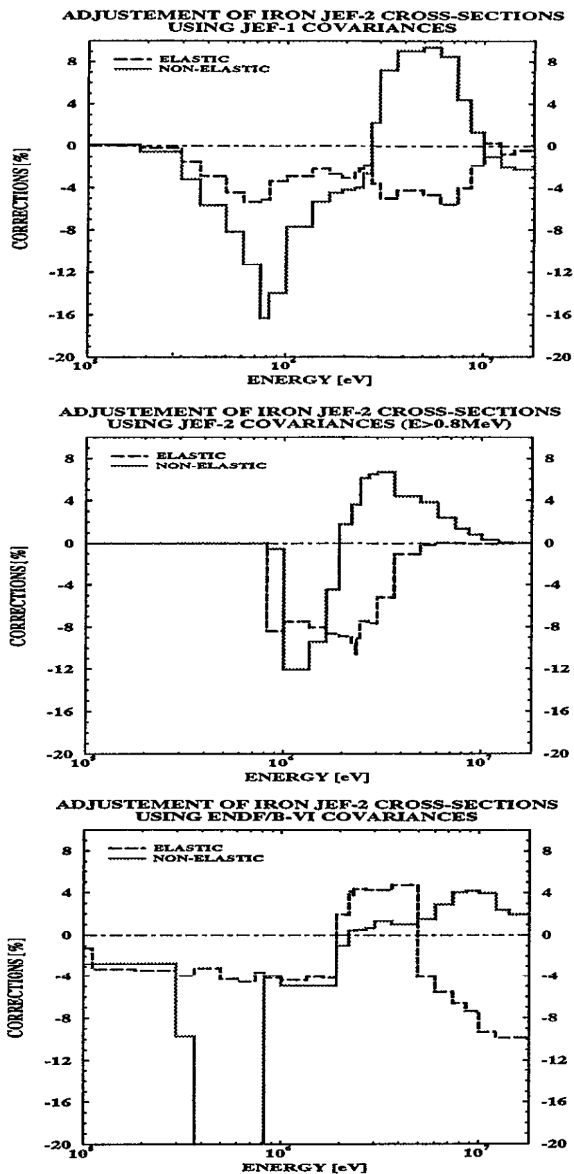
Figure 4: Adjustements of the JEF2 iron cross-sections obtained using different covariance matrices.
