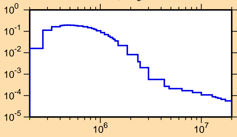
\sigma vs. E for ^{249}\text{Cf}(n,n_6)
