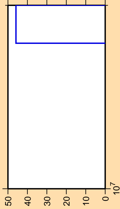
\Delta\sigma/\sigma vs. E for ^{249}\text{Cf}(n,4n)
