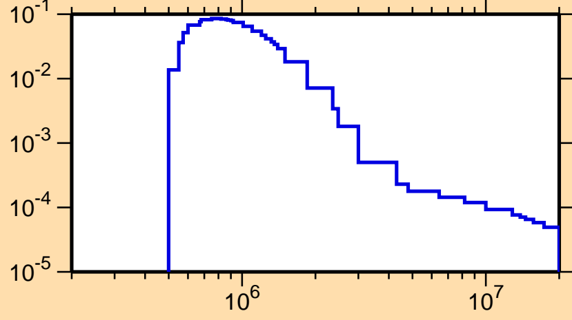
\sigma vs. E for ^{249}\text{Cf}(n,n_{17})
