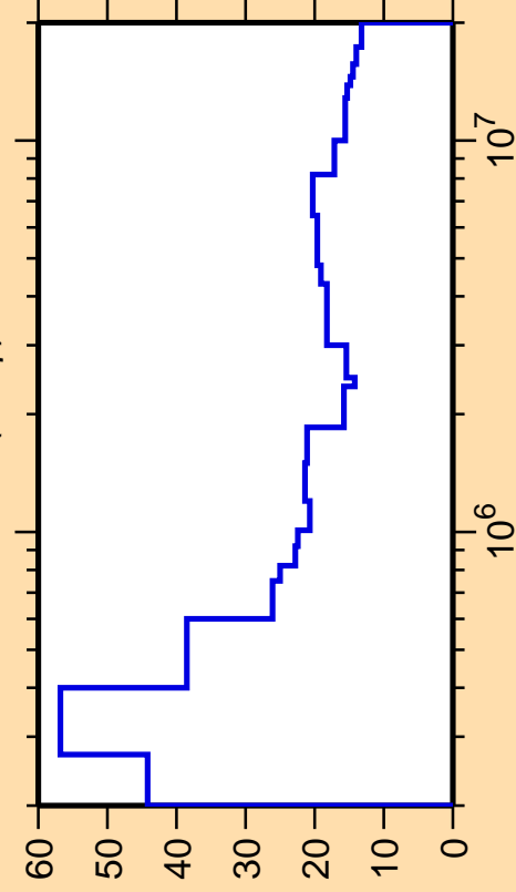
\Delta\sigma/\sigma vs. E for ^{254}\text{Es}(n,n_7)
