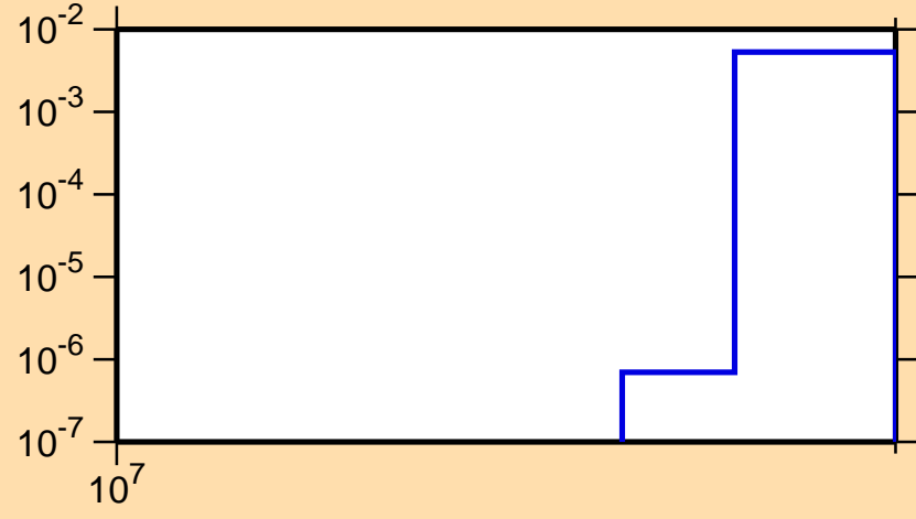
\sigma vs. E for ^{254}\text{Es}(n,4n)
