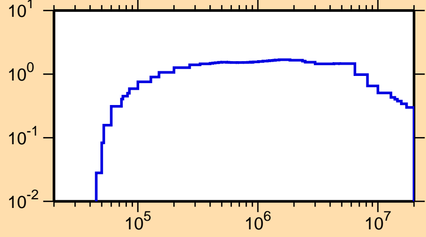
\sigma vs. E for ^{254}\text{Cf}(n,\text{inel.})
