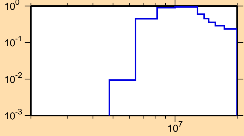
\sigma vs. E for ^{254}\text{Cf}(n,2n)
