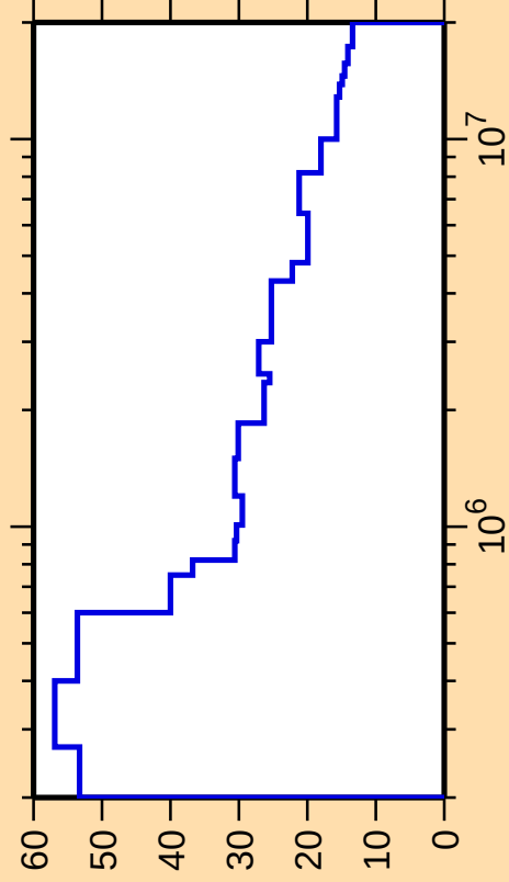
\Delta\sigma/\sigma vs. E for ^{250}\text{Bk}(n,n_{20})
