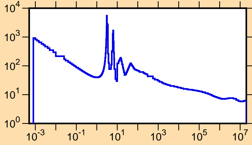
\sigma vs. E for ^{236}\text{Pu}(n,\text{tot.})
