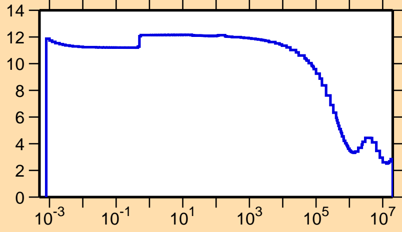
\sigma vs. E for ^{244}\text{Am}(n,\text{el.})
