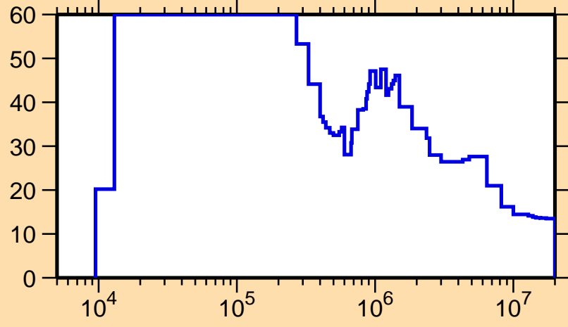
\Delta\sigma/\sigma vs. E for ^{244}\text{Am}(n,\text{inel.})
