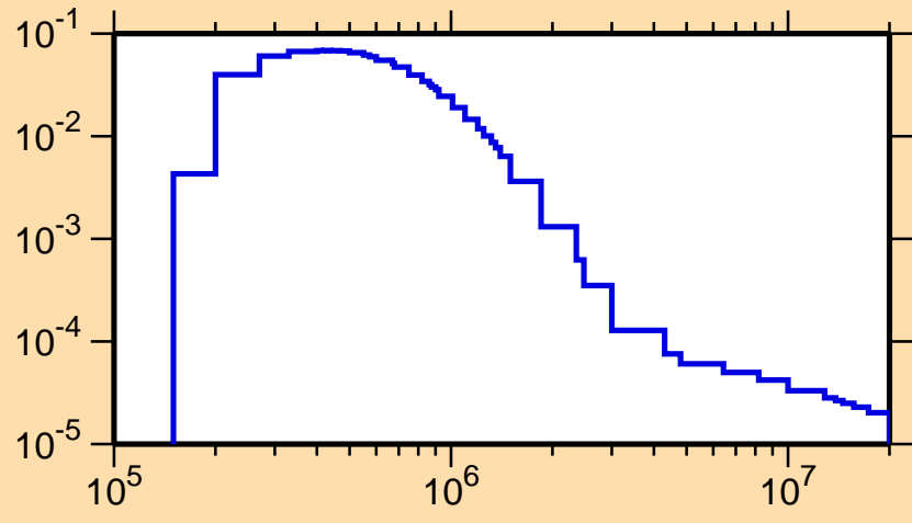
\sigma vs. E for ^{244}\text{Am}(n,n_g)
