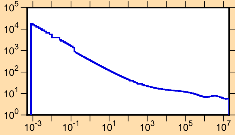
\sigma vs. E for ^{244}\text{Am}(n,\text{tot.})
