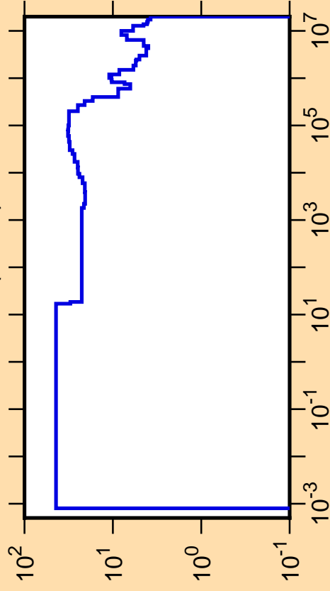
\Delta\sigma/\sigma vs. E for ^{246}\text{Pu}(n,\text{tot.})
