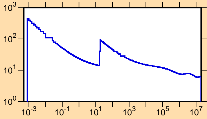
\sigma vs. E for ^{246}\text{Pu}(n,\text{tot.})
