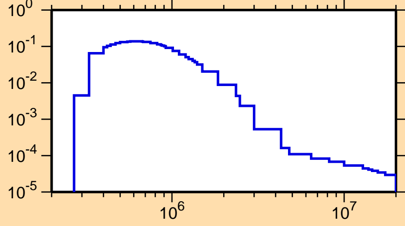
\sigma vs. E for ^{239}\text{Np}(n,n_{14})
