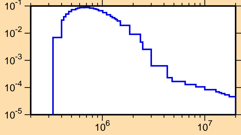
\sigma vs. E for ^{239}\text{Np}(n,n_{18})
