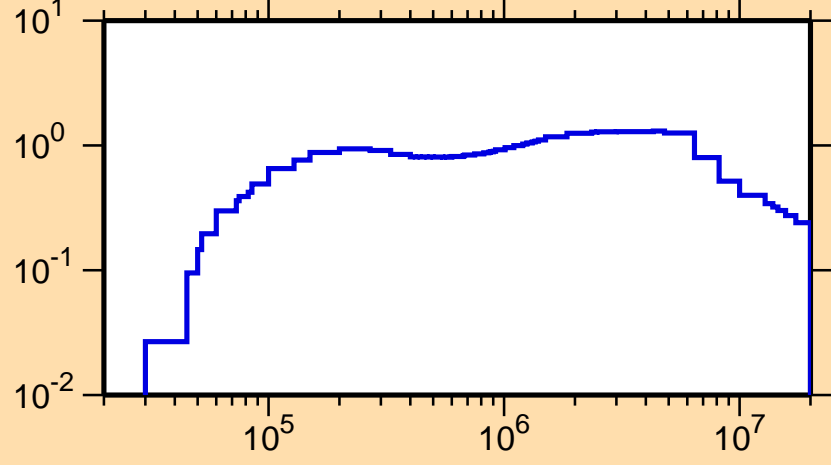
\sigma vs. E for ^{235}\text{Np}(n,\text{inel.})
