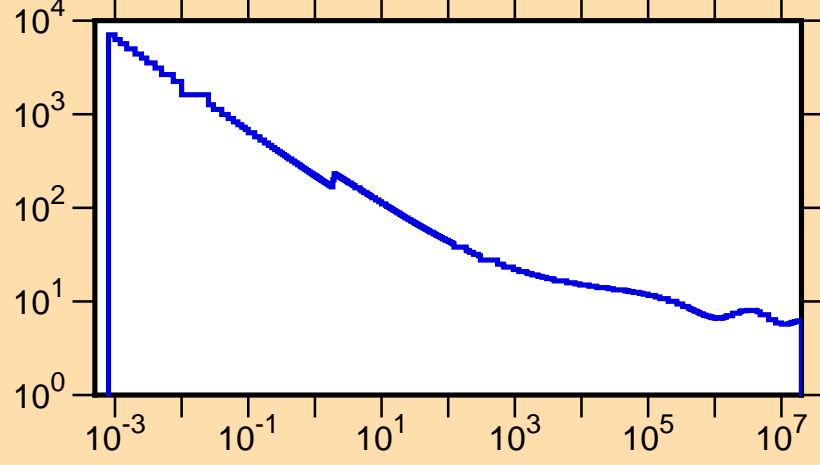
\sigma vs. E for ^{233}\text{Th}(n,\text{tot.})
