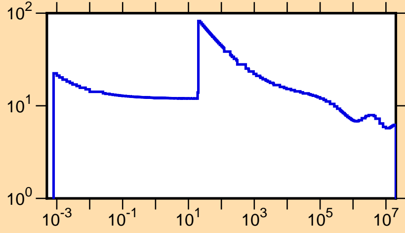
\sigma vs. E for ^{234}\text{Th}(n,\text{tot.})
