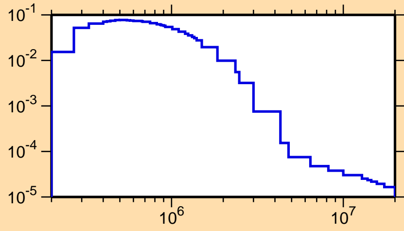
\sigma vs. E for ^{227}\text{Th}(n,n_{13})
