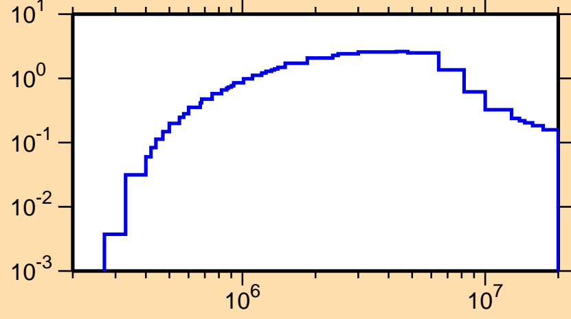
\sigma vs. E for ^{227}\text{Th}(n,n\text{cont.})
