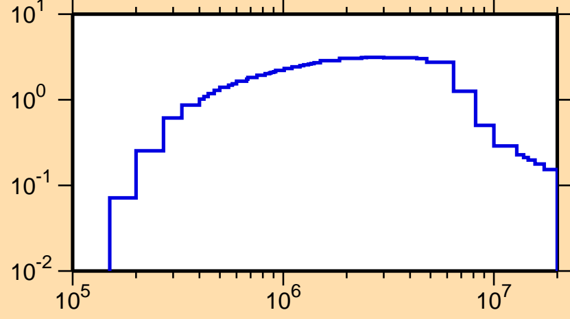
\sigma vs. E for ^{226}\text{Ac}(n,n\text{cont.})
