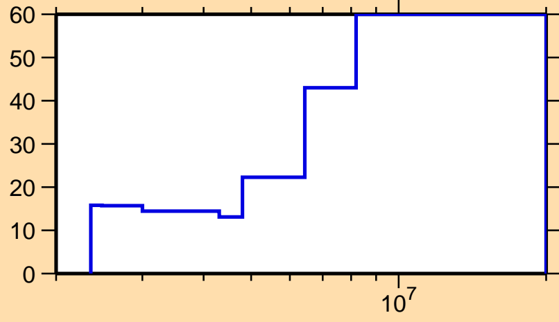
\Delta\sigma/\sigma vs. E for ^{206}\text{Pb}(n,n_6)
