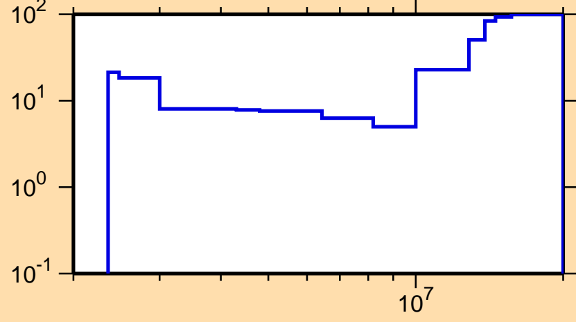
\Delta\sigma/\sigma vs. E for ^{206}\text{Pb}(n,\text{inel.})
