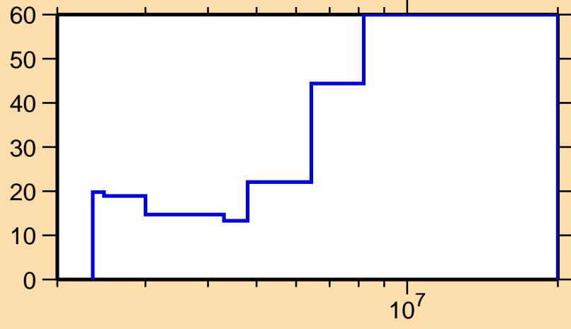
\Delta\sigma/\sigma vs. E for ^{206}\text{Pb}(n,n_7)
