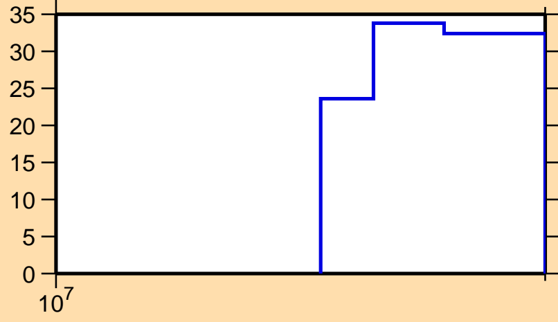
\Delta\sigma/\sigma vs. E for ^{206}\text{Pb}(n,3n)
