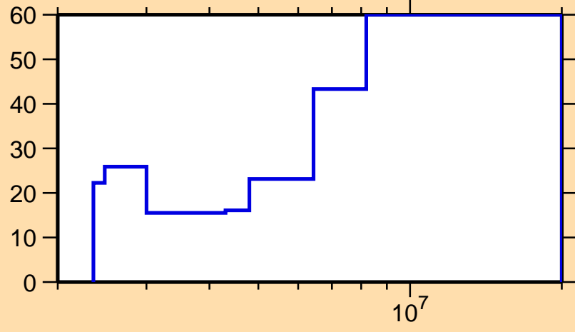
\Delta\sigma/\sigma vs. E for ^{206}\text{Pb}(n,n_{12})
