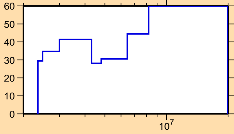
\Delta\sigma/\sigma vs. E for ^{206}\text{Pb}(n,n_{14})
