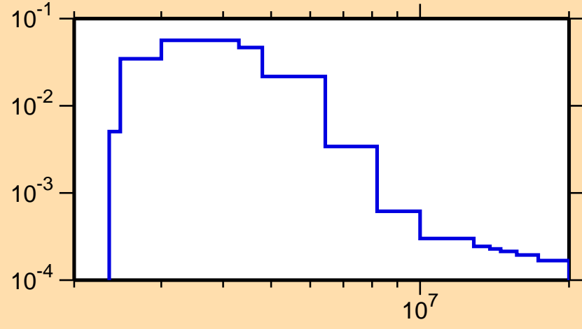
\sigma vs. E for ^{206}\text{Pb}(n,n_{15})
