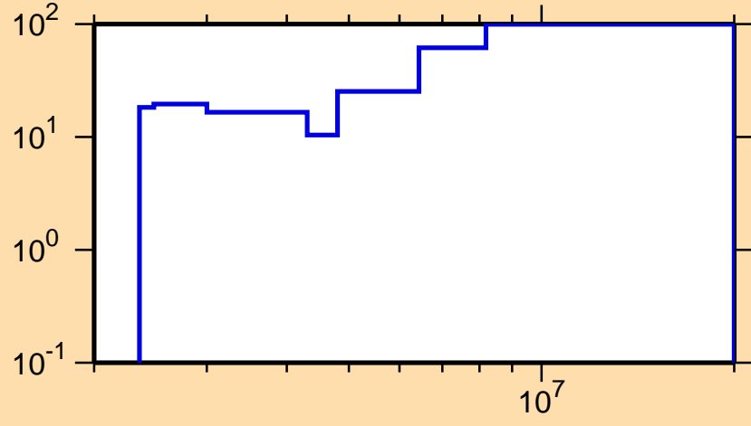
\Delta\sigma/\sigma vs. E for ^{206}\text{Pb}(n,n_2)
