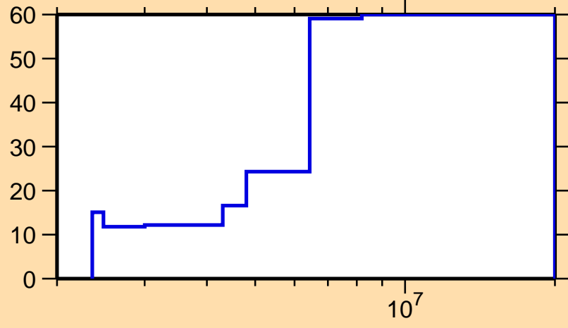
\Delta\sigma/\sigma vs. E for ^{206}\text{Pb}(n,n_{13})
