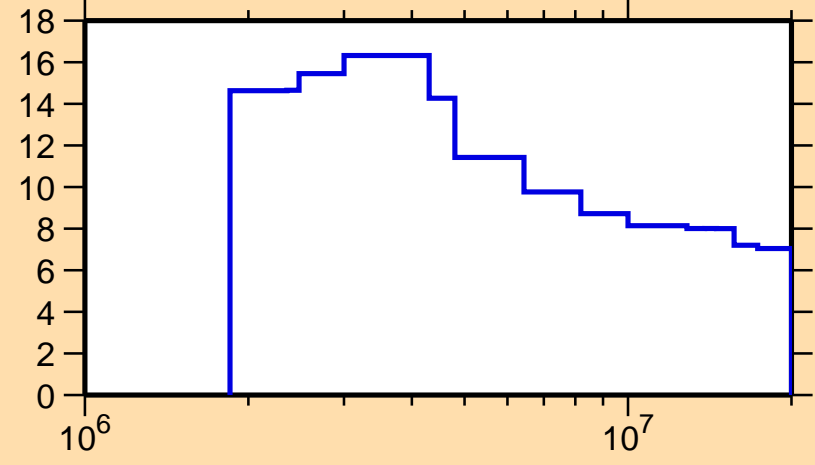
\Delta\sigma/\sigma vs. E for ^{198}\text{Hg}(n,n\text{onel.})
