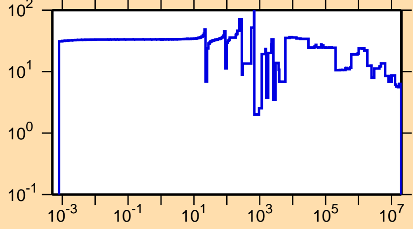
\Delta\sigma/\sigma vs. E for ^{198}\text{Hg}(n,\text{el.})
