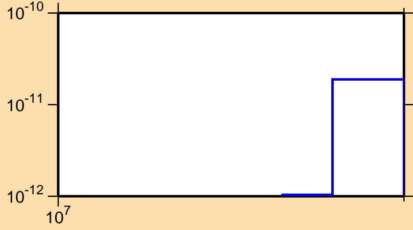
\sigma vs. E for ^{198}\text{Hg}(n,p\alpha)
