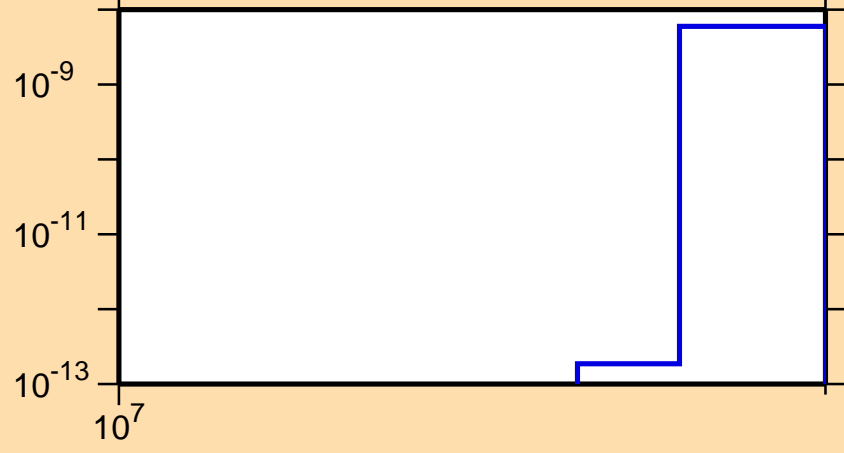
\sigma vs. E for ^{198}\text{Hg}(n,nt)
