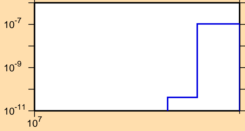
\sigma vs. E for ^{198}\text{Hg}(n,\text{nd})
