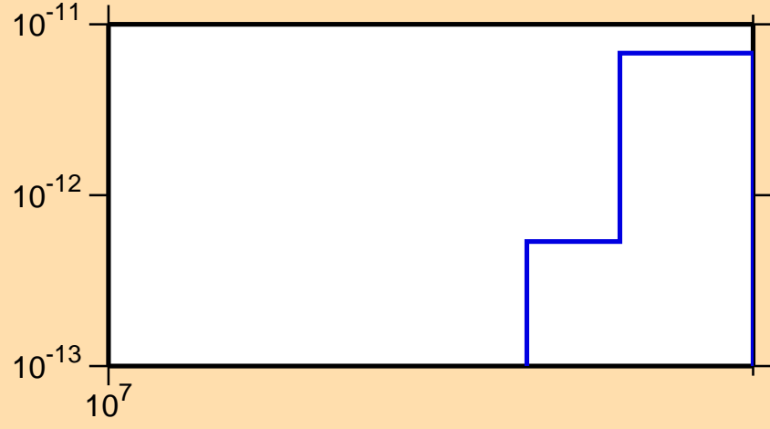
\sigma vs. E for ^{199}\text{Hg}(n,p\alpha)
