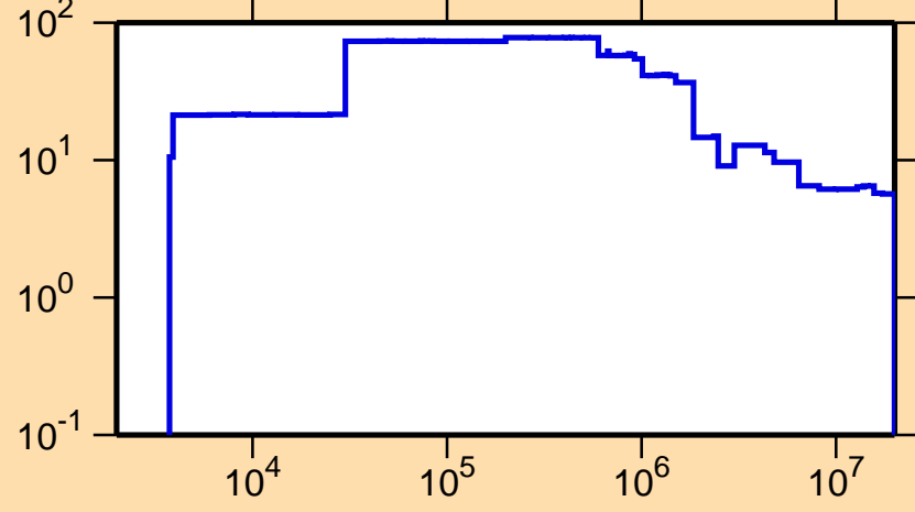
\Delta\sigma/\sigma vs. E for ^{199}\text{Hg}(n,\text{nonel.})
