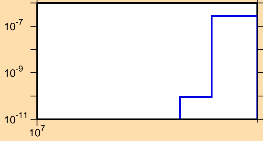
\sigma vs. E for ^{199}\text{Hg}(n,2np)
