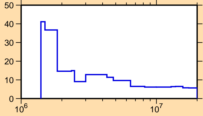
\Delta\sigma/\sigma vs. E for ^{199}\text{Hg}(n,n\text{onel.})
