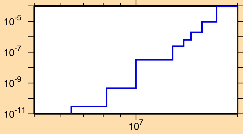
\sigma vs. E for ^{198}\text{Pt}(n,\alpha)
