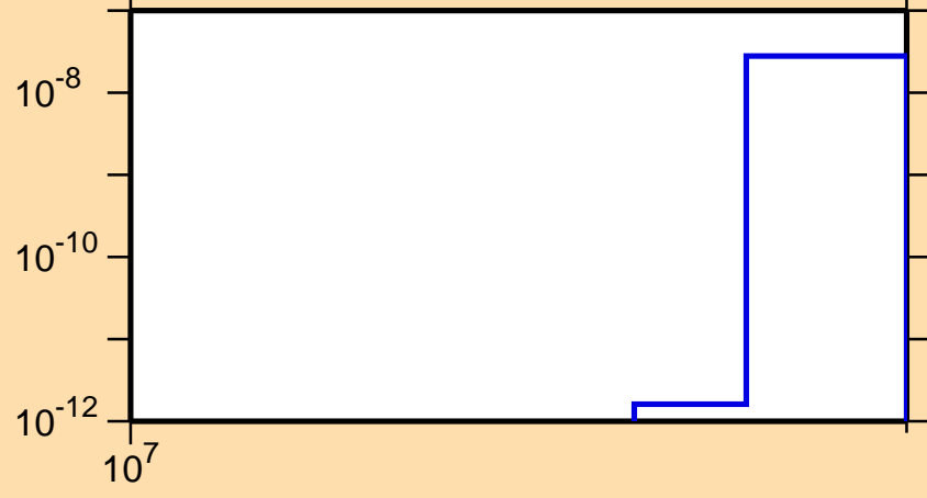
\sigma vs. E for ^{198}\text{Pt}(n,nt)
