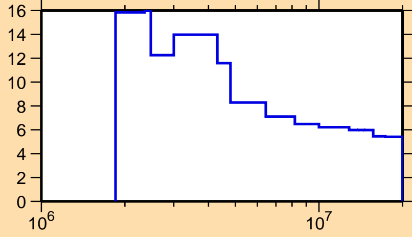
\Delta\sigma/\sigma vs. E for ^{198}\text{Pt}(n,n\text{onel.})
