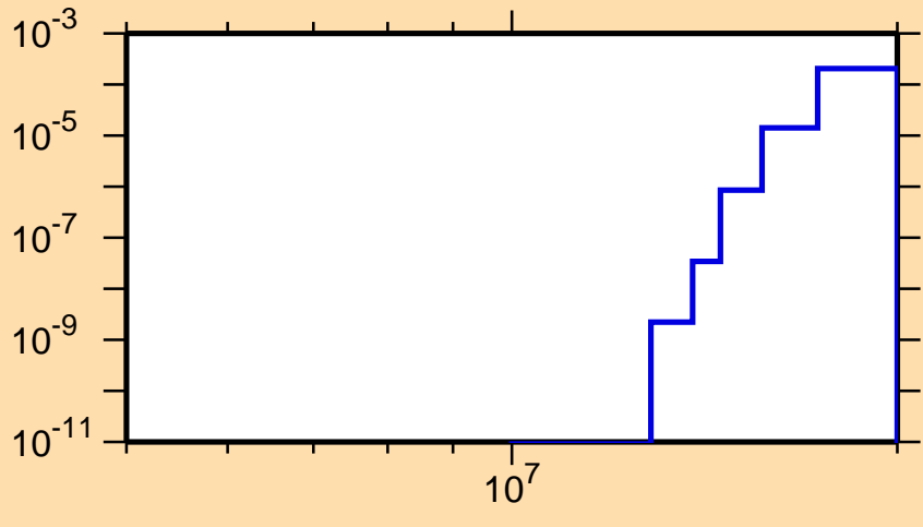
\sigma vs. E for ^{198}\text{Pt}(n,t)
