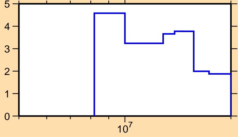
\Delta\sigma/\sigma vs. E for ^{190}\text{Pt}(n,\text{tot.})
