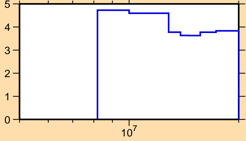
\Delta\sigma/\sigma vs. E for ^{190}\text{Pt}(n,\text{nonel.})
