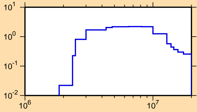
\sigma vs. E for ^{190}\text{Pt}(n,n\text{cont.})
