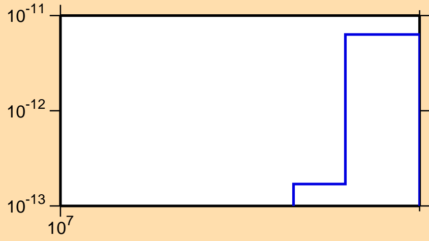
\sigma vs. E for ^{190}\text{Ir} (mt 45)
