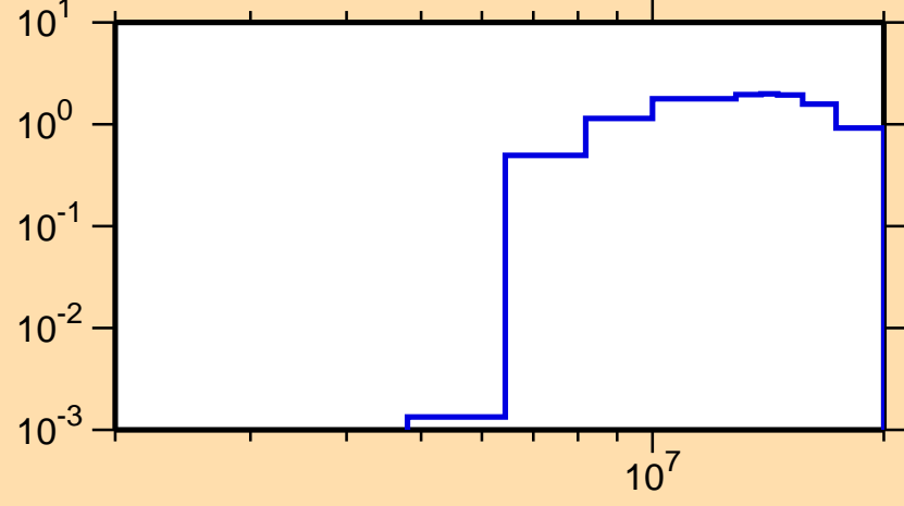
\sigma vs. E for ^{192}\text{Ir}(n,2n)
