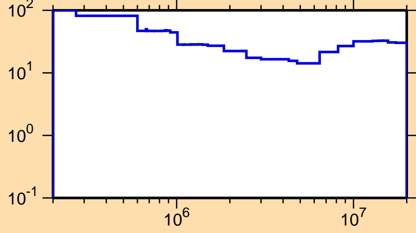
\Delta\sigma/\sigma vs. E for ^{192}\text{Ir}(n,n\text{cont.})
