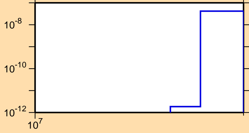
\sigma vs. E for ^{190}\text{Os}(n,2np)
