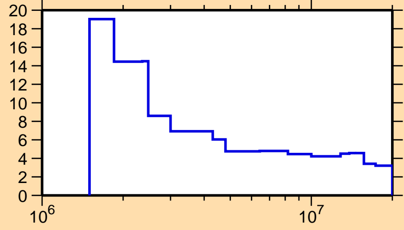
\Delta\sigma/\sigma vs. E for ^{190}\text{Os}(n,n\text{onel.})
