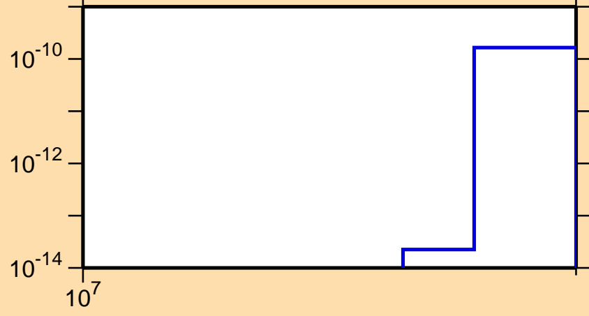
\sigma vs. E for ^{190}\text{Os}(n,3n\alpha)
