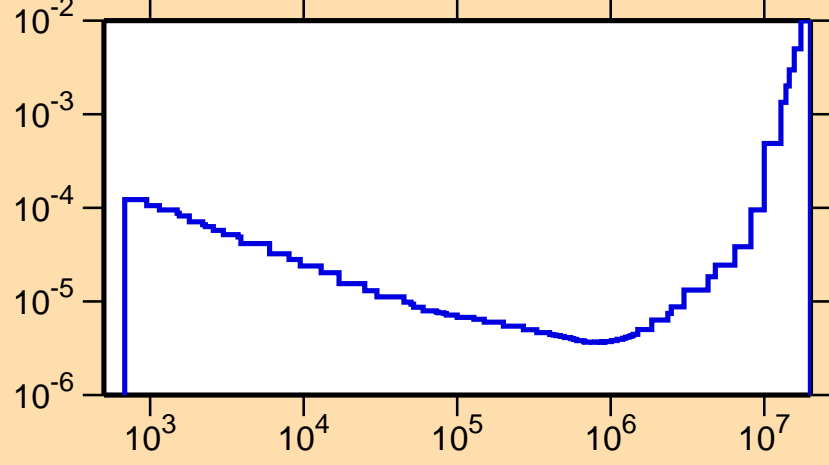
\sigma vs. E for ^{191}\text{Pt}(n,\alpha)
