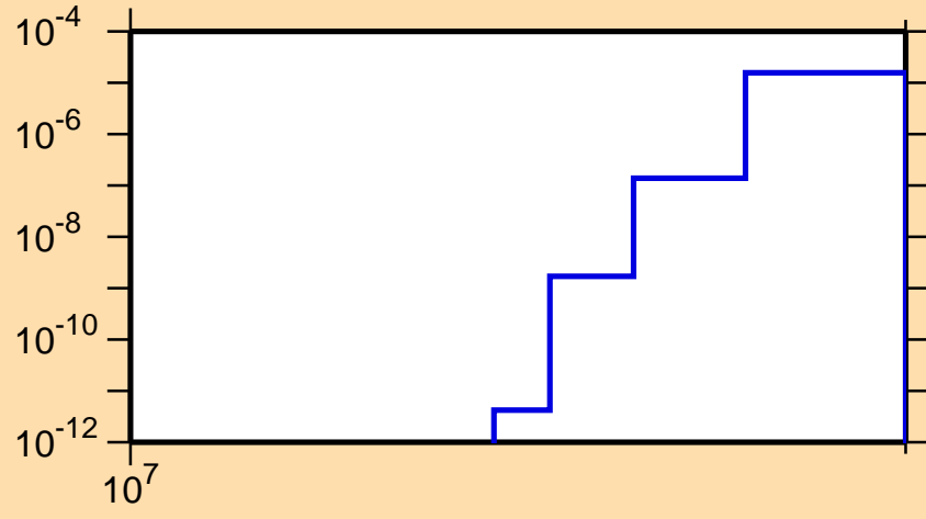
\sigma vs. E for ^{191}\text{Pt}(n,\text{nd})
