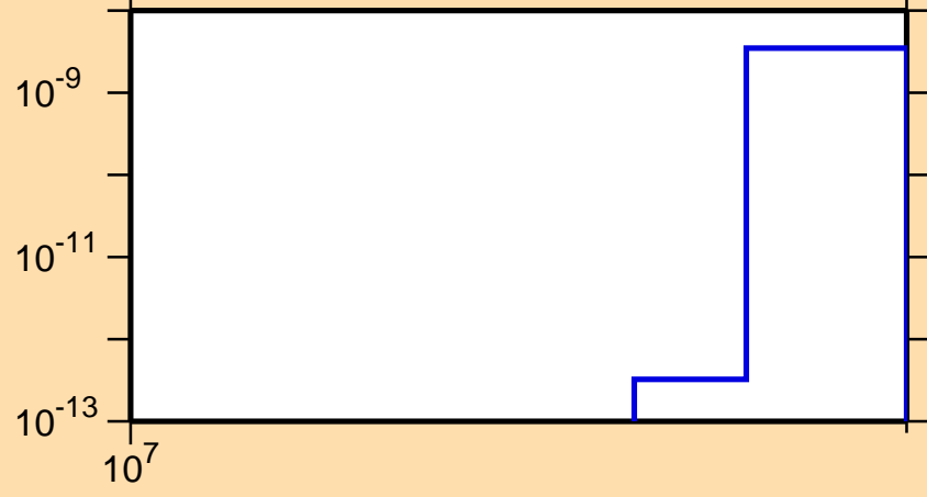
\sigma vs. E for ^{191}\text{Pt}(n,3n\alpha)
