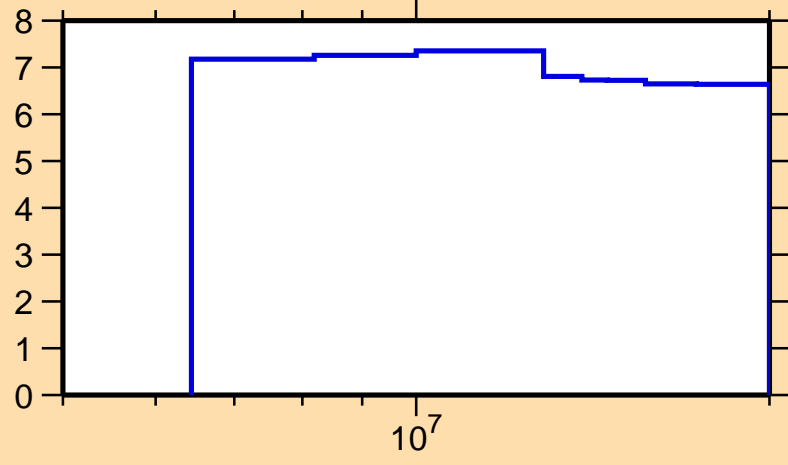
\Delta\sigma/\sigma vs. E for ^{191}\text{Pt}(n,\text{nonel.})
