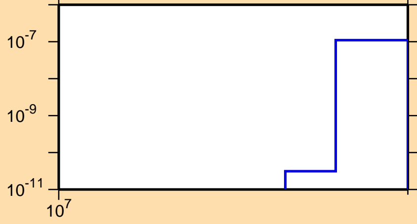
\sigma vs. E for ^{191}\text{Pt}(n,nt)
