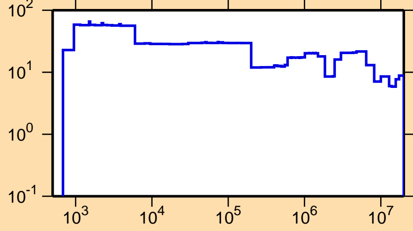
\Delta\sigma/\sigma vs. E for ^{191}\text{Pt}(n,\text{el.})
