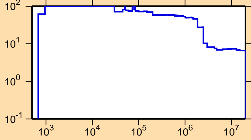
\Delta\sigma/\sigma vs. E for ^{191}\text{Pt}(n,\text{nonel.})
