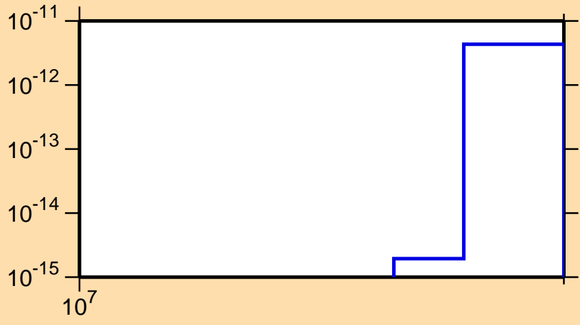
\sigma vs. E for ^{191}\text{Pt}(\text{mt } 34)
