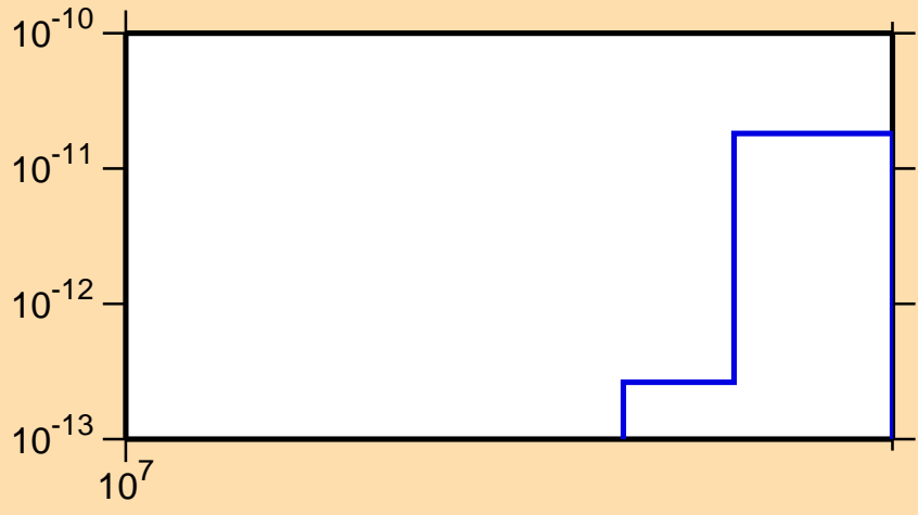
\sigma vs. E for ^{191}\text{Pt}(\text{mt } 45)
