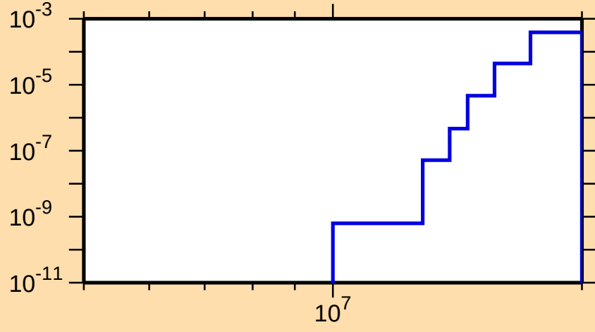
\sigma vs. E for ^{193}\text{Os}(n,t)
