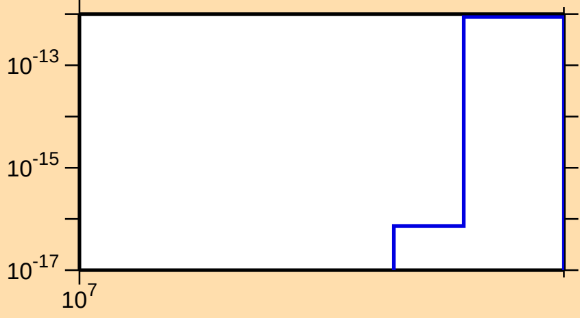
\sigma vs. E for ^{193}\text{Os}(n,3n\alpha)
