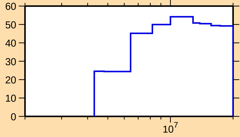
\Delta\sigma/\sigma vs. E for ^{193}\text{Os}(n,n\text{cont.})
