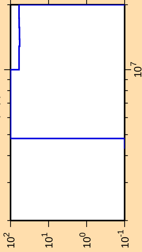
\Delta\sigma/\sigma vs. E for ^{193}\text{Os}(n,p)
