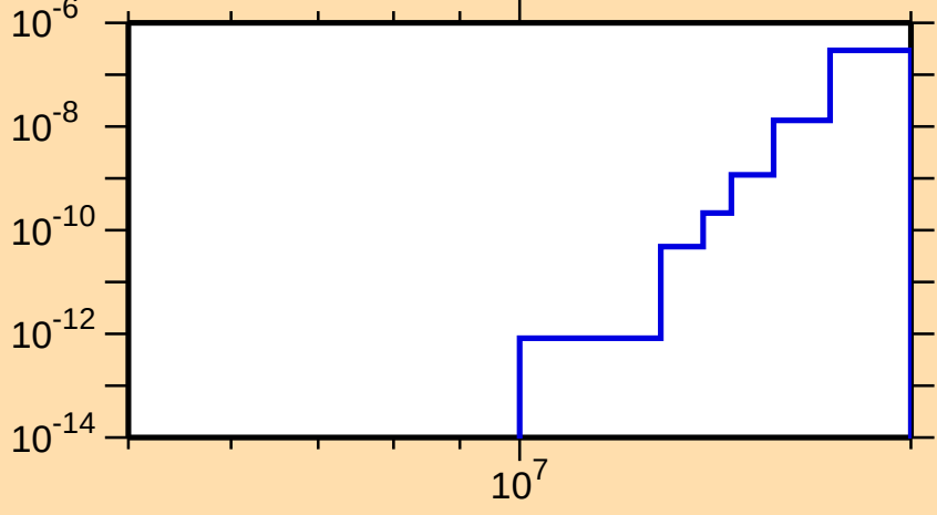
\sigma vs. E for ^{193}\text{Os}(n,2n\alpha)
