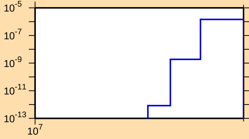
\sigma vs. E for ^{193}\text{Os}(n,\text{nd})
