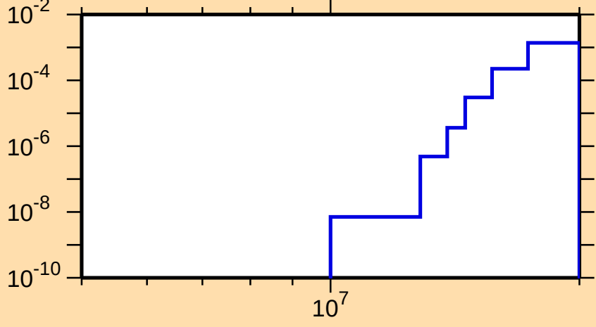
\sigma vs. E for ^{193}\text{Os}(n,d)
