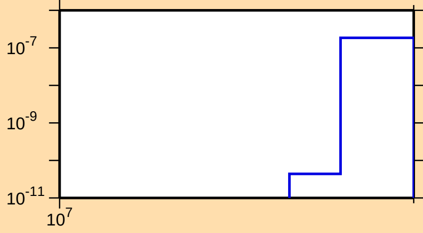
\sigma vs. E for ^{193}\text{Os}(n,2np)
