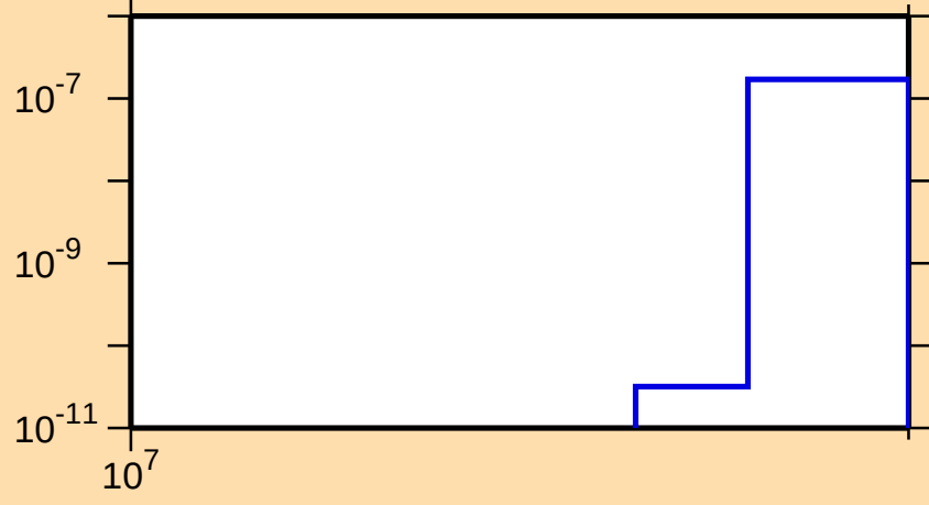
\sigma vs. E for ^{193}\text{Os}(n,nt)
