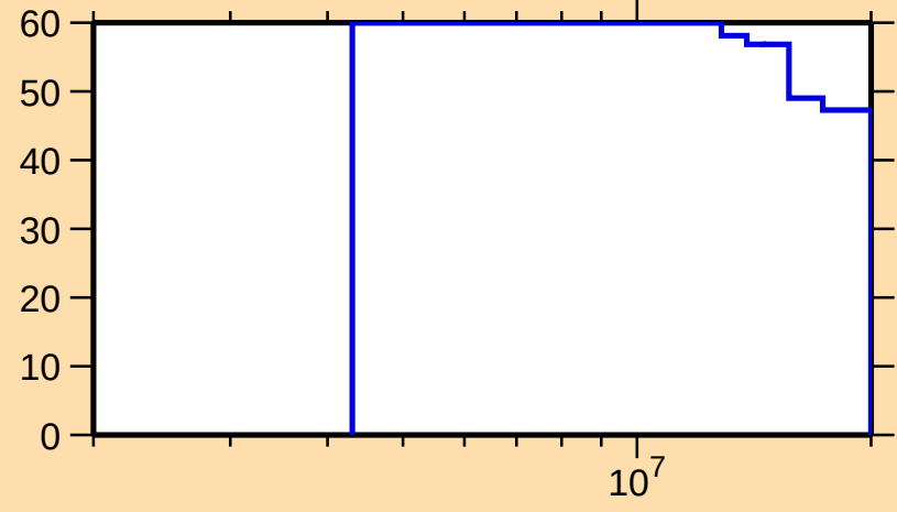
\Delta\sigma/\sigma vs. E for ^{193}\text{Os}(n,\gamma)
