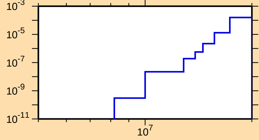
\sigma vs. E for ^{193}\text{Os}(n,n\alpha)
