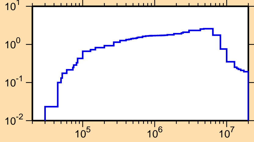
\sigma vs. E for ^{189}\text{Os}(n,\text{inel.})
