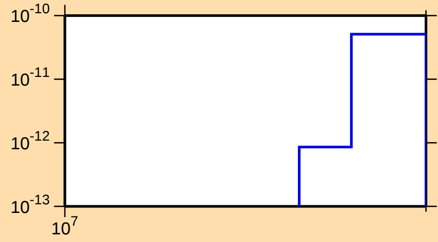
\sigma vs. E for ^{186}\text{Os}(\text{mt117})
