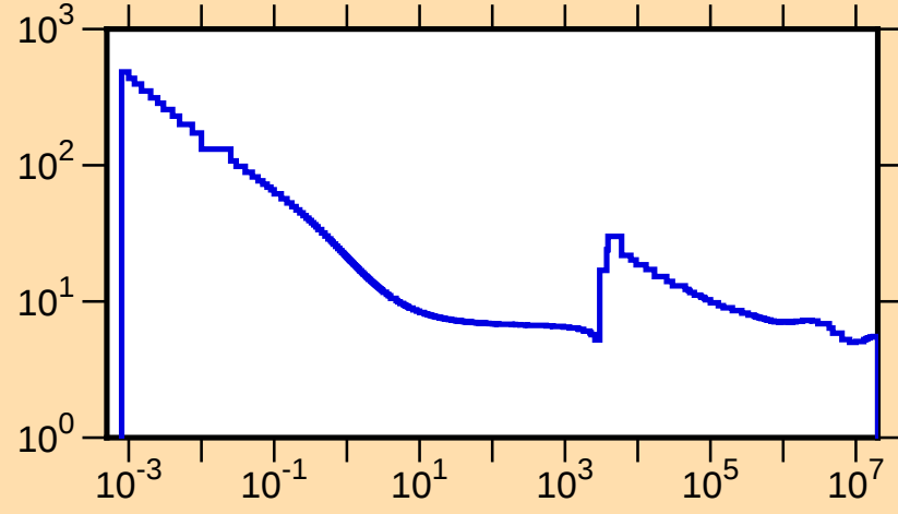
\sigma vs. E for ^{186}\text{Os}(n,\text{tot.})
