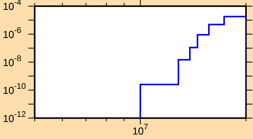
\sigma vs. E for ^{186}\text{Os}(n,2n\alpha)
