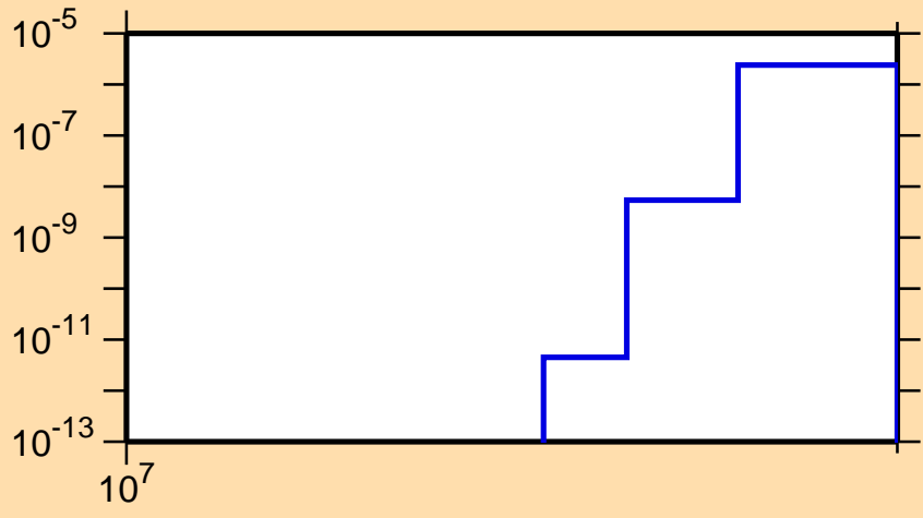
\sigma vs. E for ^{193}\text{Pt}(n,2np)
