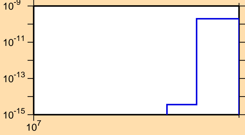
\sigma vs. E for ^{193}\text{Pt}(n,3n\alpha)
