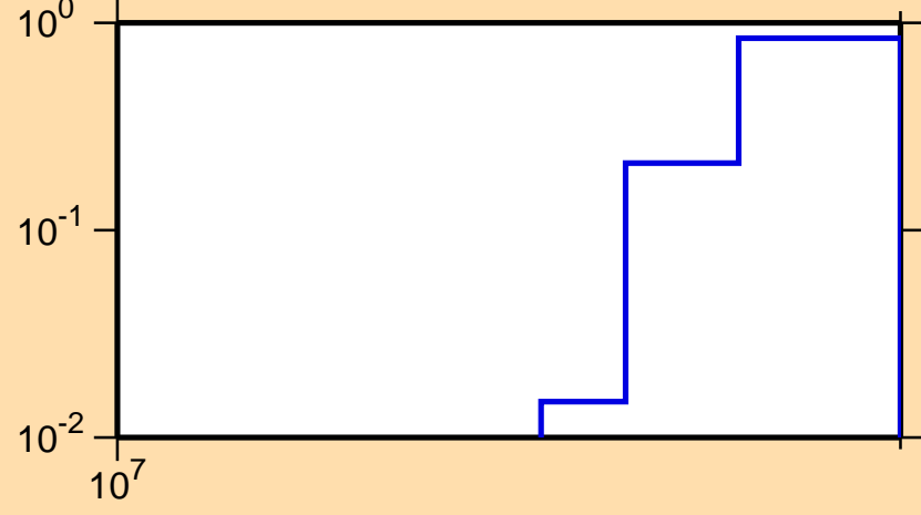
\sigma vs. E for ^{193}\text{Pt}(n,3n)
