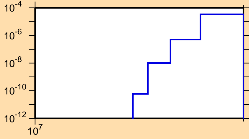
\sigma vs. E for ^{185}\text{Os}(n,\text{nd})
