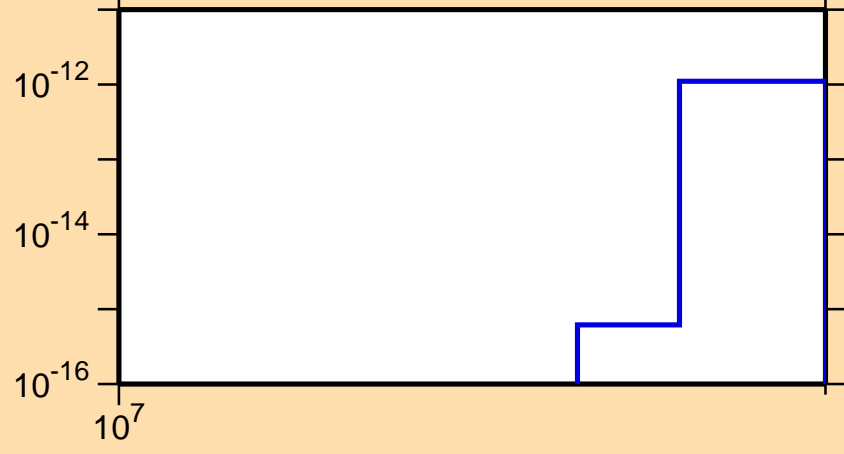
\sigma vs. E for ^{185}\text{Os}(n,\text{pt})
