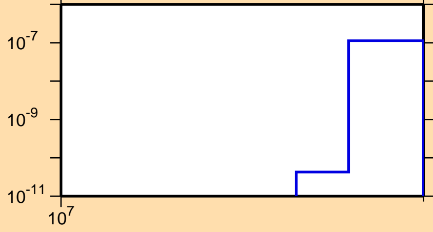
\sigma vs. E for ^{185}\text{Os}(n,nt)
