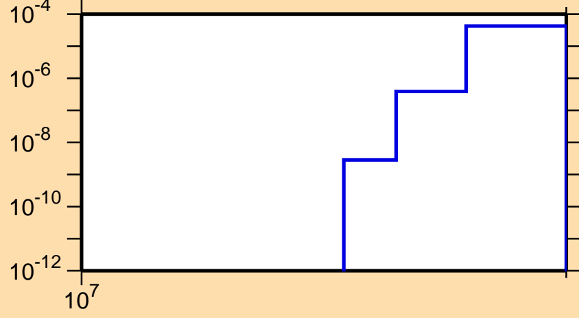
\sigma vs. E for ^{185}\text{Os}(n,2np)
