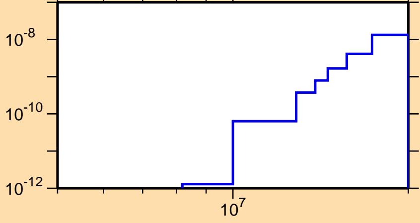
\sigma vs. E for ^{185}\text{Os}(n,p\alpha)
