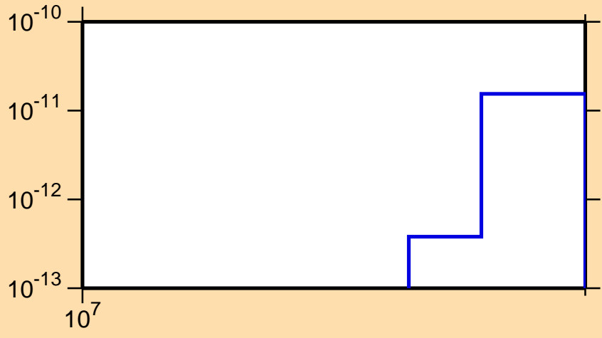
\sigma vs. E for ^{185}\text{Os}(\text{mt117})
