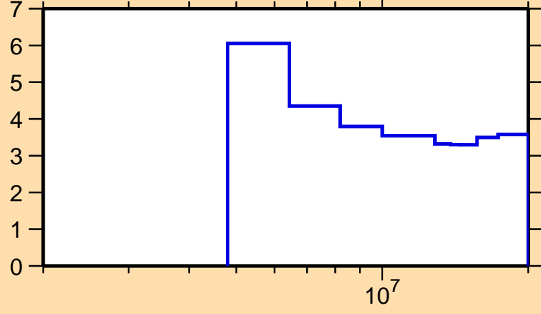
\Delta\sigma/\sigma vs. E for ^{186}\text{Re}(n,\text{nonel.})
