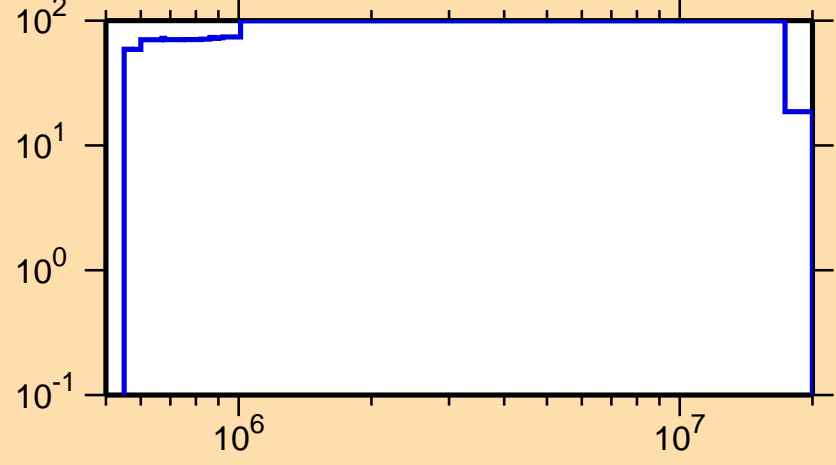
\Delta\sigma/\sigma vs. E for ^{186}\text{Re}(n,n_1)
