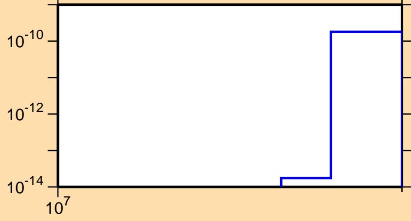
\sigma vs. E for ^{186}\text{Re}(n,3n\alpha)
