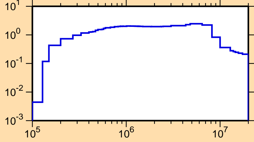
\sigma vs. E for ^{177}\text{Lu}(n,\text{inel.})
