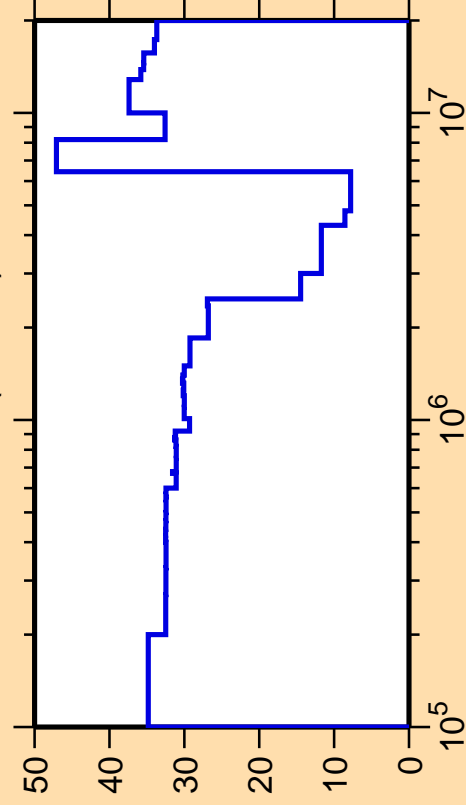
\Delta\sigma/\sigma vs. E for ^{177}\text{Lu}(n,\text{inel.})
