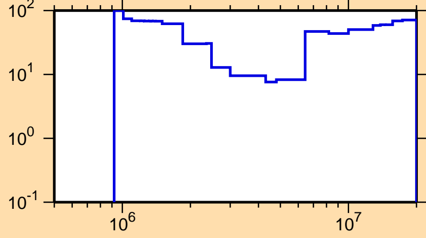
\Delta\sigma/\sigma vs. E for ^{177}\text{Lu}(n,n\text{cont.})
