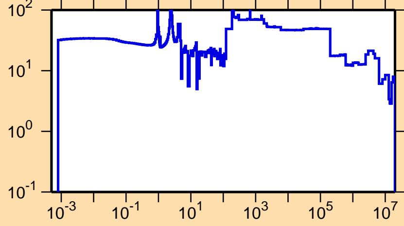
\Delta\sigma/\sigma vs. E for ^{177}\text{Lu}(n,\text{el.})
