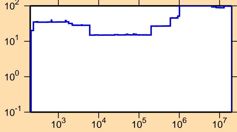
\Delta\sigma/\sigma vs. E for ^{180}\text{Ta}(n,\gamma)
