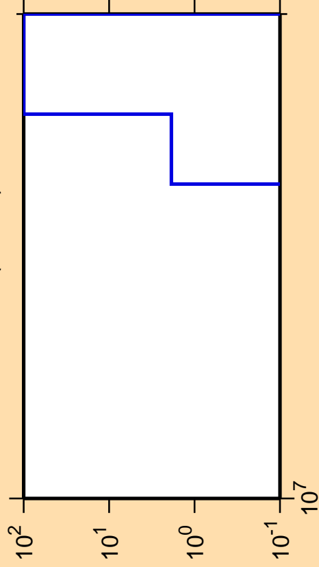
\Delta\sigma/\sigma vs. E for ^{180}\text{Ta} (mt 45)
