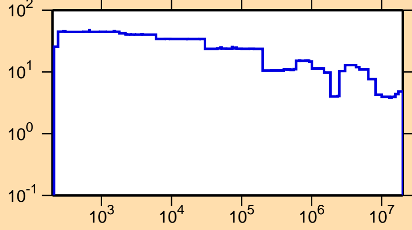
\Delta\sigma/\sigma vs. E for ^{180}\text{Ta}(n,\text{tot.})
