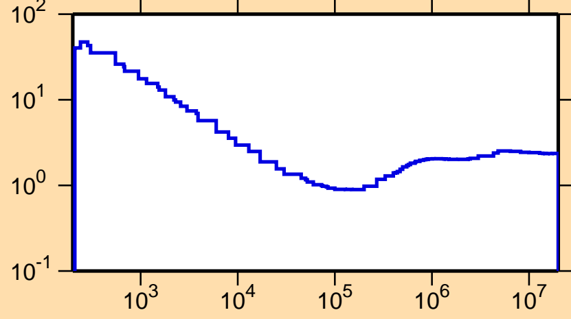
\sigma vs. E for ^{180}\text{Ta}(n,\text{nonel.})
