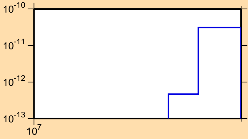
\sigma vs. E for ^{180}\text{Ta} (mt 45)
