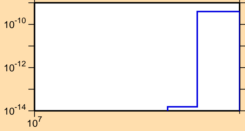
\sigma vs. E for ^{180}\text{Ta}(n,3n\alpha)
