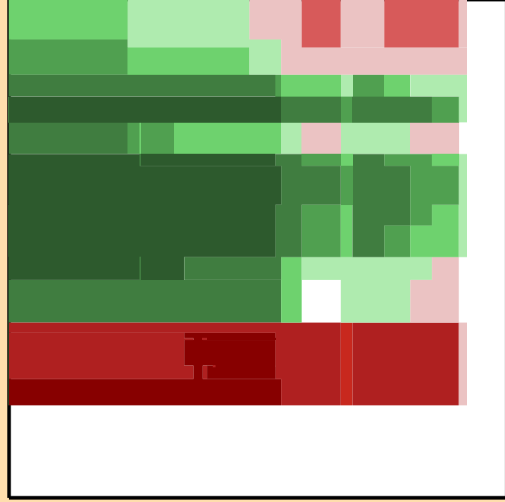
\Delta\sigma/\sigma vs. E for ^{180}\text{Ta}(n,n_1)
