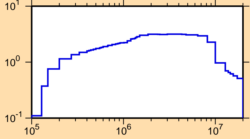
\sigma vs. E for ^{180}\text{W}(n,\text{inel.})
