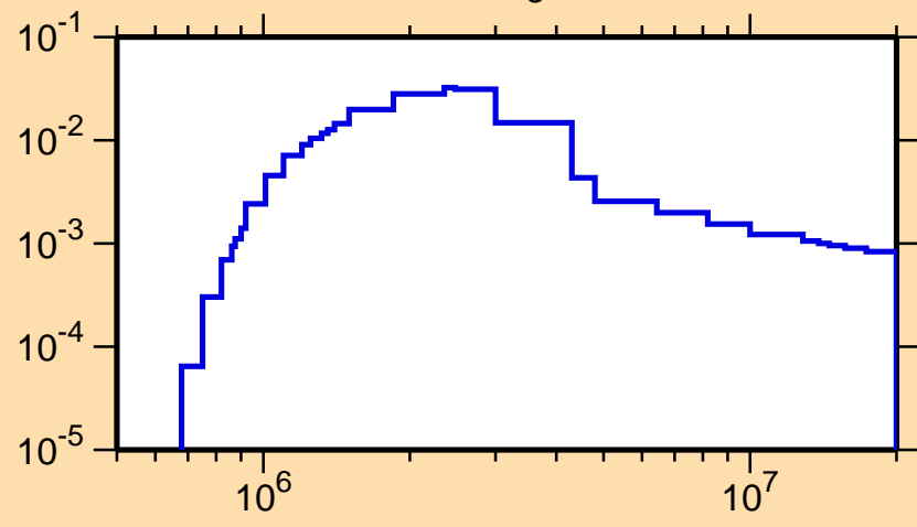
\sigma vs. E for ^{180}\text{W}(n,n_3)
