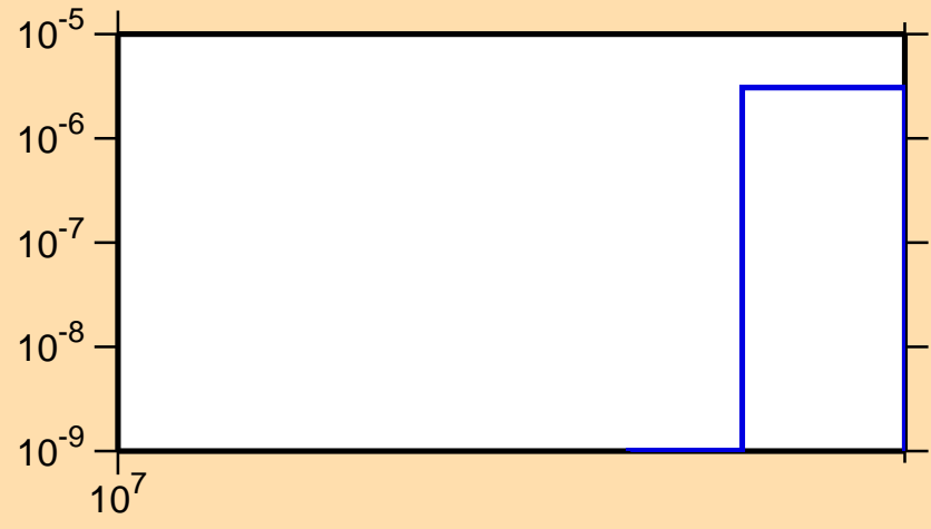
\sigma vs. E for ^{180}\text{W}(n,2np)
