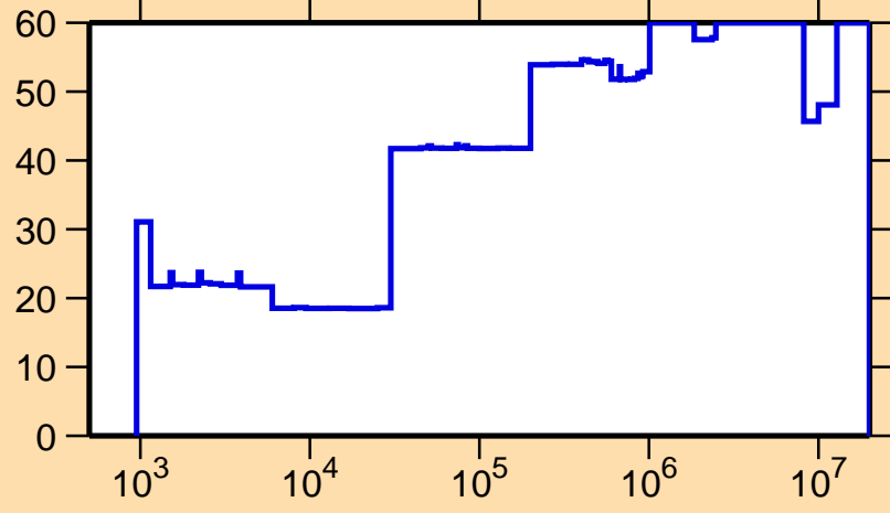
\Delta\sigma/\sigma vs. E for ^{180}\text{W}(n,\gamma)
