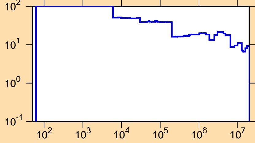
\Delta\sigma/\sigma vs. E for ^{182}\text{Ta}(n,\text{el.})
