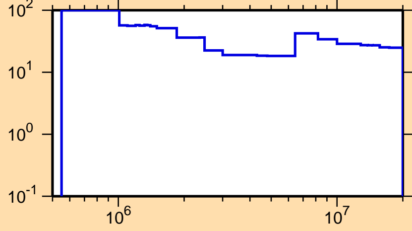
\Delta\sigma/\sigma vs. E for ^{182}\text{Ta}(n,n\text{cont.})
