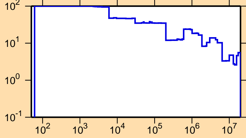
\Delta\sigma/\sigma vs. E for ^{182}\text{Ta}(n,\text{tot.})
