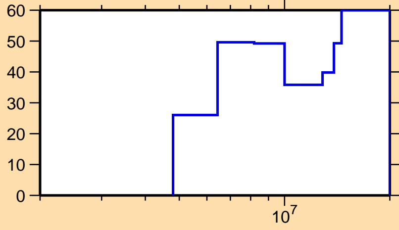
\Delta\sigma/\sigma vs. E for ^{179}\text{Hf}(n,\gamma)
