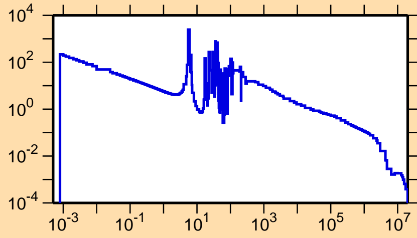
\sigma vs. E for ^{179}\text{Hf}(n,\gamma)
