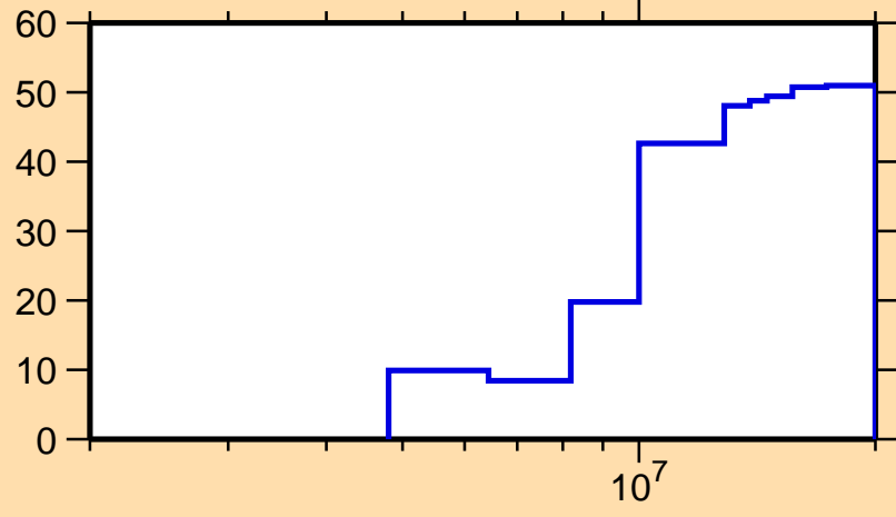
\Delta\sigma/\sigma vs. E for ^{179}\text{Hf}(n,\text{inel.})
