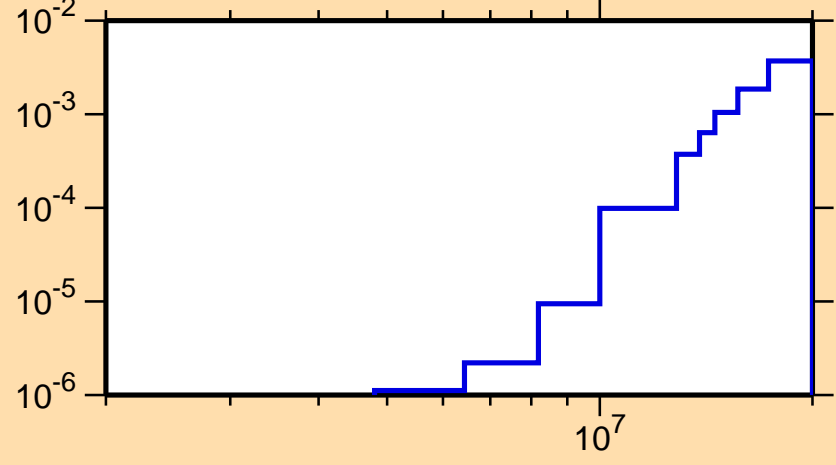
\sigma vs. E for ^{179}\text{Hf}(n,\alpha)
