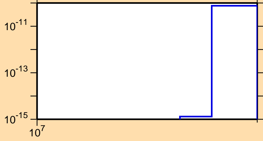
\sigma vs. E for ^{173}\text{Lu}(n,3n\alpha)
