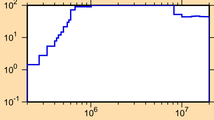
\Delta\sigma/\sigma vs. E for ^{173}\text{Lu}(n,p)
