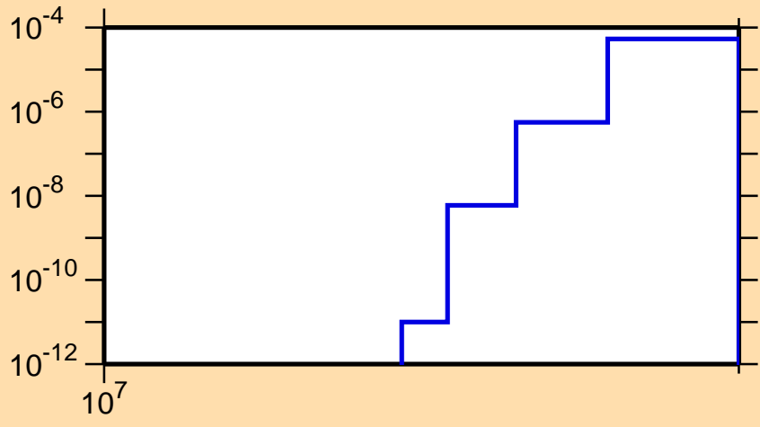
\sigma vs. E for ^{173}\text{Lu}(n,nd)
