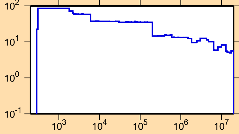
\Delta\sigma/\sigma vs. E for ^{173}\text{Lu}(n,\text{el.})
