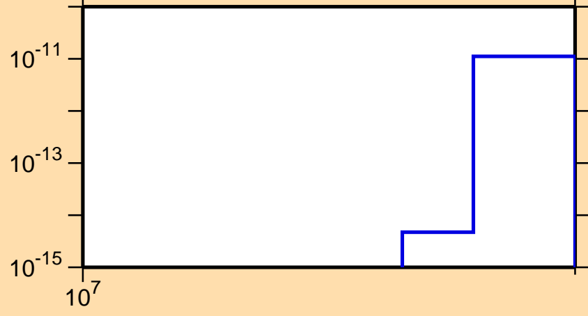
\sigma vs. E for ^{176}\text{Yb}(n,\text{He3})
