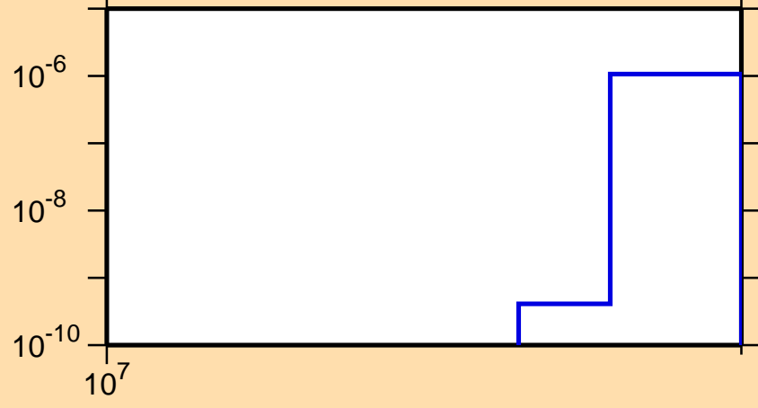
\sigma vs. E for ^{173}\text{Yb}(n,nt)
