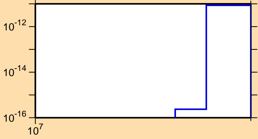
\sigma vs. E for ^{173}\text{Yb}(n,3n\alpha)
