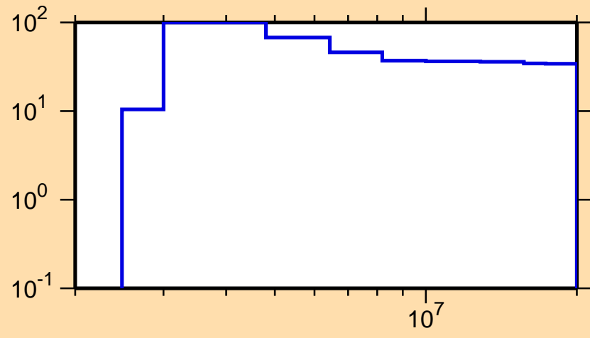
\Delta\sigma/\sigma vs. E for ^{173}\text{Yb}(n,p)
