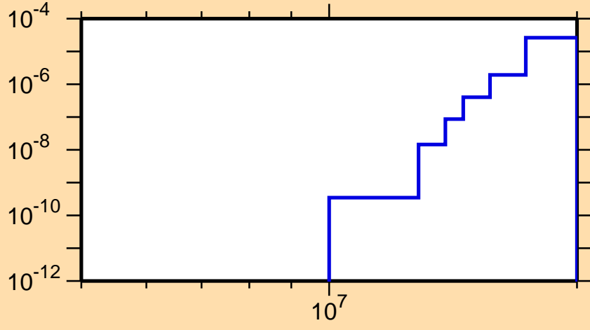
\sigma vs. E for ^{173}\text{Yb}(n,2n\alpha)
