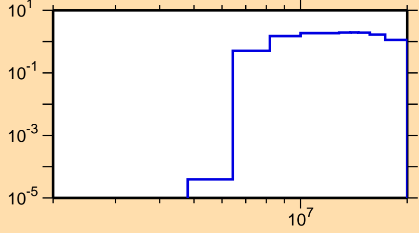
\sigma vs. E for ^{173}\text{Yb}(n,2n)
