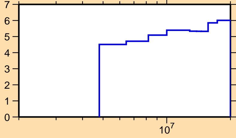
\Delta\sigma/\sigma vs. E for ^{173}\text{Yb}(n,\text{nonel.})
