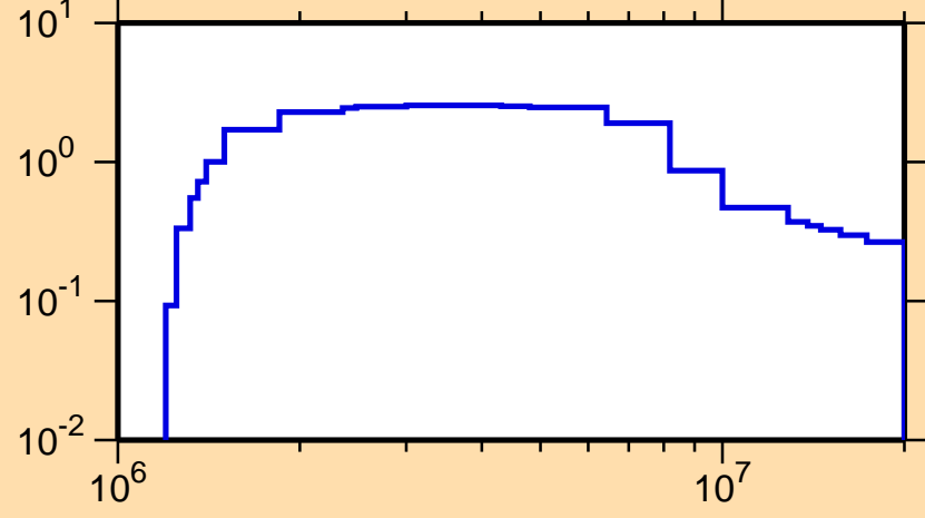
\sigma vs. E for ^{173}\text{Yb}(n,n\text{cont.})
