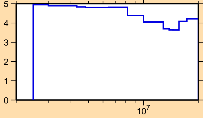
\Delta\sigma/\sigma vs. E for ^{172}\text{Yb}(n,\text{nonel.})
