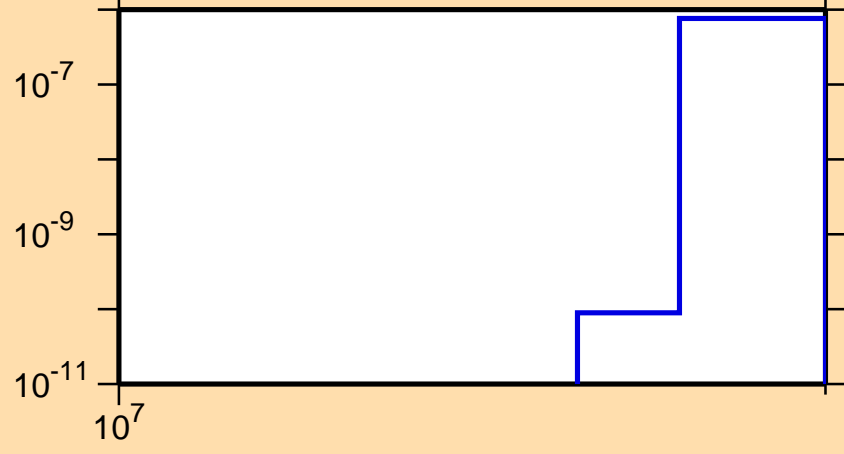
\sigma vs. E for ^{172}\text{Yb}(n,2np)
