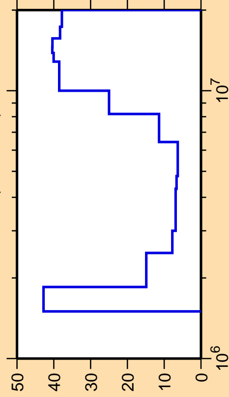
\Delta\sigma/\sigma vs. E for ^{172}\text{Yb}(n,\text{ncont.})
