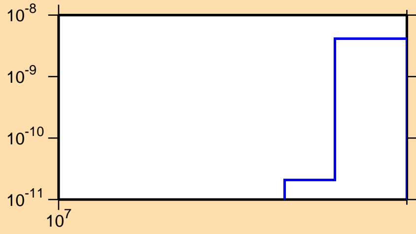
\sigma vs. E for ^{172}\text{Yb}(n,\text{He3})
