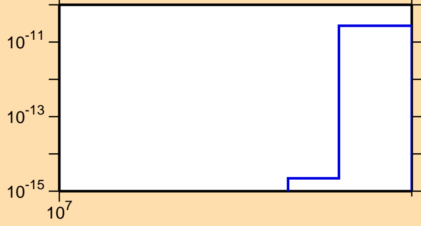
\sigma vs. E for ^{172}\text{Yb}(n,3n\alpha)
