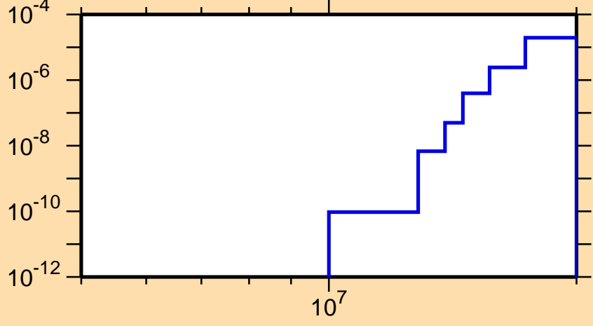
\sigma vs. E for ^{159}\text{Dy}(n,2n\alpha)
