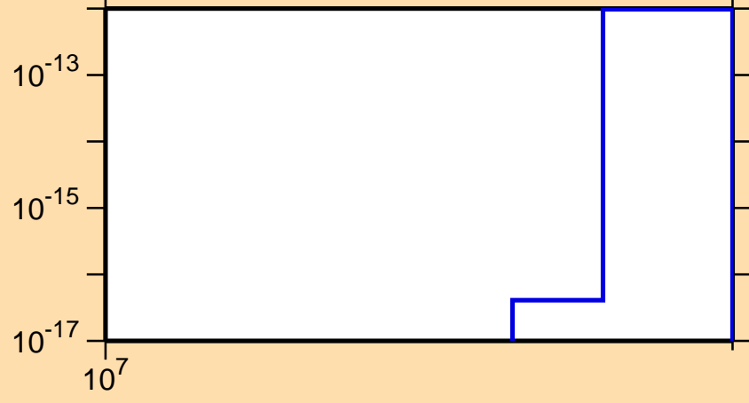
\sigma vs. E for ^{159}\text{Dy} (mt 34)
