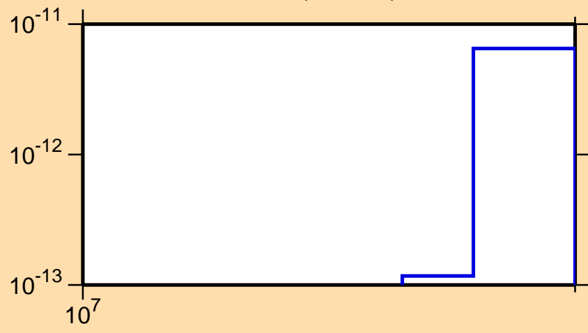
\sigma vs. E for ^{169}\text{Yb}(\text{mt117})
